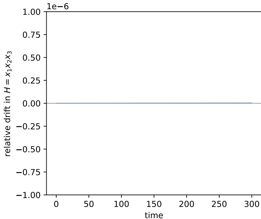
Invariant conserved (max drift 2.3\text{e-}09 )
