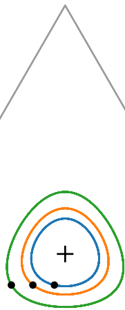
Closed orbits about (1/3, 1/3, 1/3)
