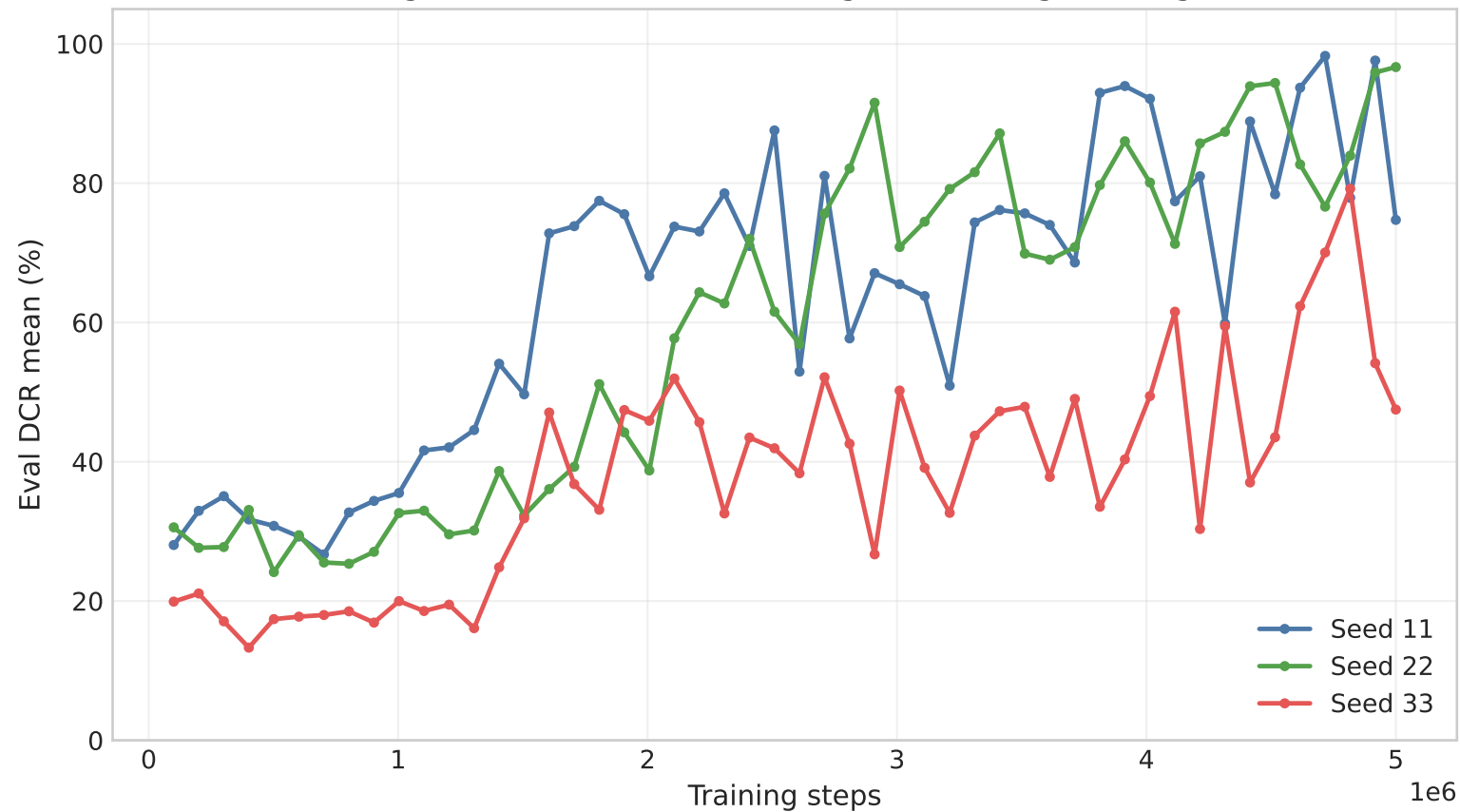
Figure 2: PPO full seed divergence during training
