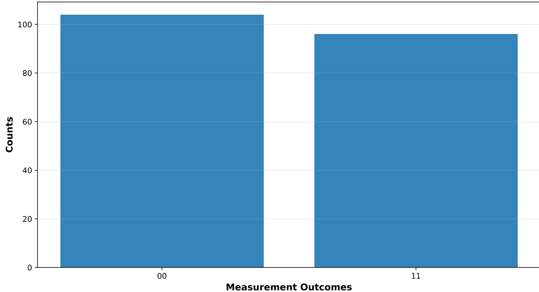
GHZ State - (2 qubits)
