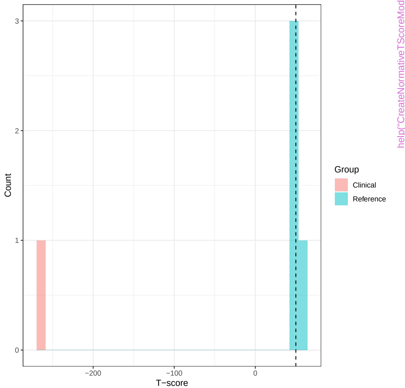
T-score distribution
