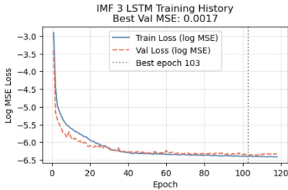
FIG. 7: Training and validation MSE loss curves per epoch for K = 3 IMF's LSTM, from the GA-VMD-LSTM. Loss is plotted on a log scale. Vertical line at epoch 103 shows the best model checkpoint.
