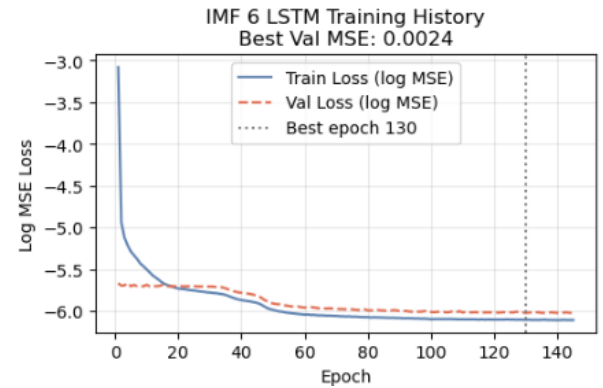
FIG. 10: Training and validation MSE loss curves per epoch for K = 6 IMF's LSTM, from the GA-VMD-LSTM. Loss is plotted on a log scale. Vertical line at epoch 130 shows the best model checkpoint.
