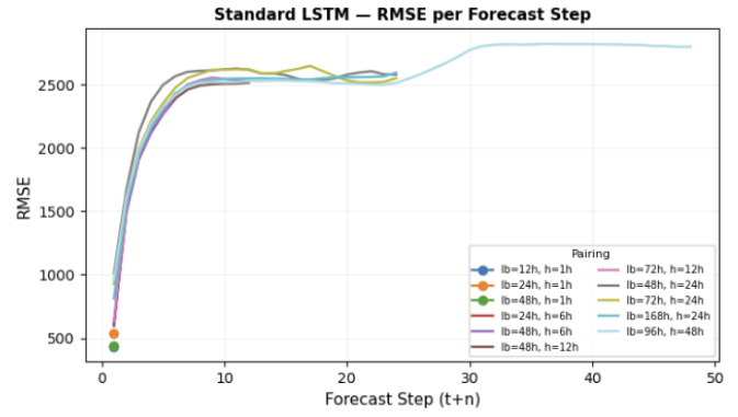
FIG. 15: Investigation of the effects of various (lookback, horizon) pairings on the baseline LSTM's RMSE performance per predictive step.
