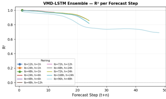
FIG. 4: Investigation of the effects of various (lookback, horizon) pairings on the GA-VMD-LSTM Ensemble’s R^2 performance per predictive step. Modelling is of station SQ19.
