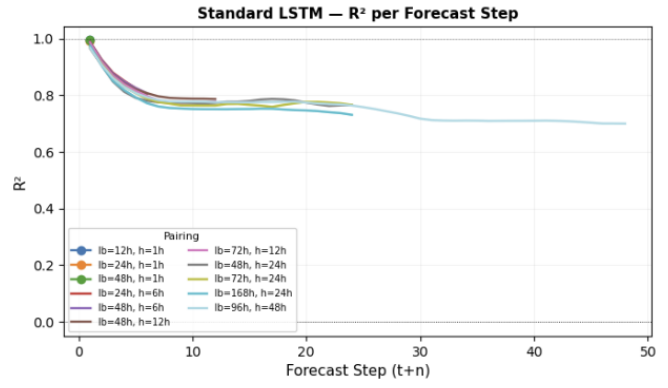
FIG. 14: Investigation of the effects of various (lookback, horizon) pairings on the baseline LSTM's R^2 performance per predictive step.
