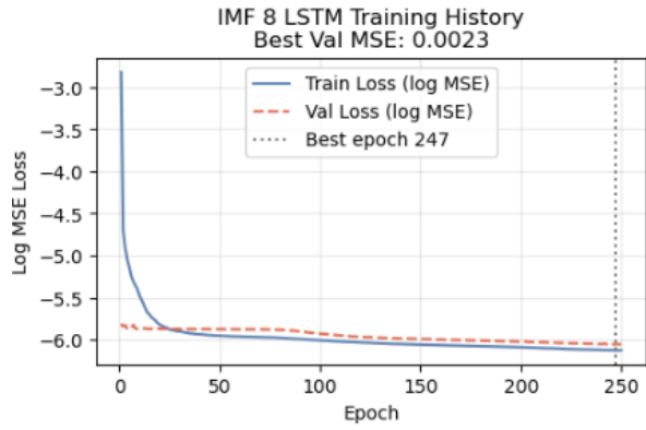
FIG. 12: Training and validation MSE loss curves per epoch for K = 8 IMF's LSTM, from the GA-VMD-LSTM. Loss is plotted on a log scale. Vertical line at epoch 247 shows the best model check-point.
