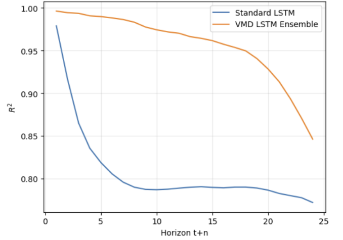
FIG. 1: Line plot of R^2 between model predictions and actual test set values across the full horizon for both the baseline LSTM and the GA-VMD-LSTM Ensemble. Modelling is of station SQ19.
