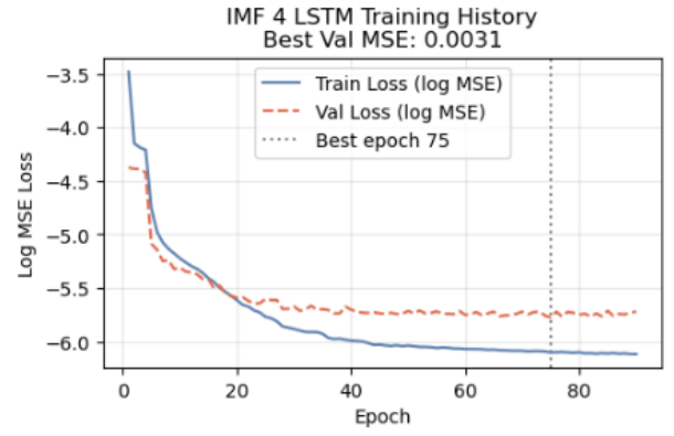
FIG. 8: Training and validation MSE loss curves per epoch for K = 4 IMF's LSTM, from the GA-VMD-LSTM. Loss is plotted on a log scale. Vertical line at epoch 75 shows the best model checkpoint.
