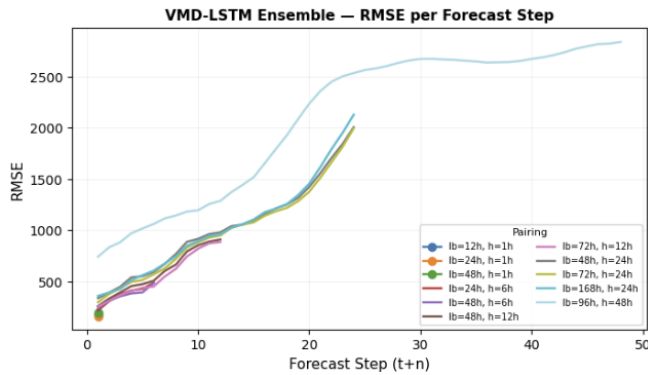
FIG. 13: Investigation of the effects of various (lookback, horizon) pairings on the GA-VMD-LSTM Ensemble's RMSE performance per predictive step.
