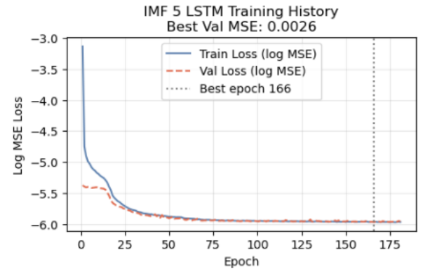
FIG. 9: Training and validation MSE loss curves per epoch for K = 5 IMF's LSTM, from the GA-VMD-LSTM. Loss is plotted on a log scale. Vertical line at epoch 166 shows the best model checkpoint.
