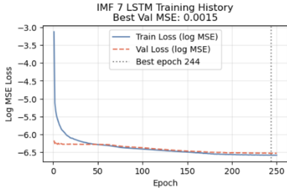
FIG. 11: Training and validation MSE loss curves per epoch for K = 7 IMF's LSTM, from the GA-VMD-LSTM. Loss is plotted on a log scale. Vertical line at epoch 244 shows the best model check-point.
