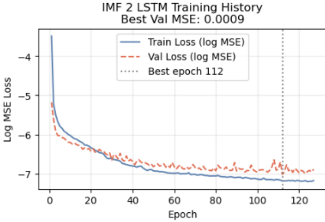
FIG. 3: Training and validation MSE loss curves per epoch for K = 2 IMF's LSTM, from the GA-VMD-LSTM. Loss is plotted on a log scale. Vertical line at epoch 112 shows the best model checkpoint. Modelling is of station SQ19.
