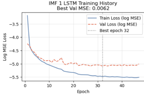
FIG. 6: Training and validation MSE loss curves per epoch for K = 1 IMF's LSTM, from the GA-VMD-LSTM. Loss is plotted on a log scale. Vertical line at epoch 32 shows the best model checkpoint.
