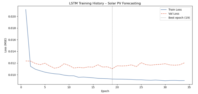
FIG. 2: Training and validation MSE loss curves per epoch for baseline LSTM. Vertical line at epoch 19 shows the best model checkpoint. Modelling is of station SQ19.
