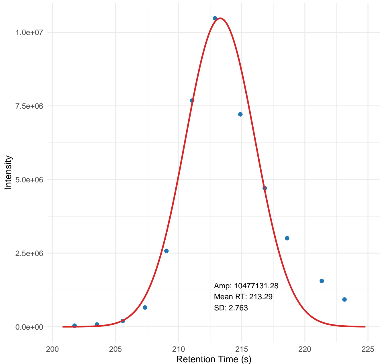
Gaussian Peak Fit – Suspect 1(mz = 283.175)
