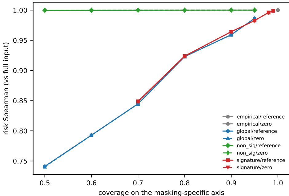
A. Coverage \rightarrow risk stability (three masking arms)
