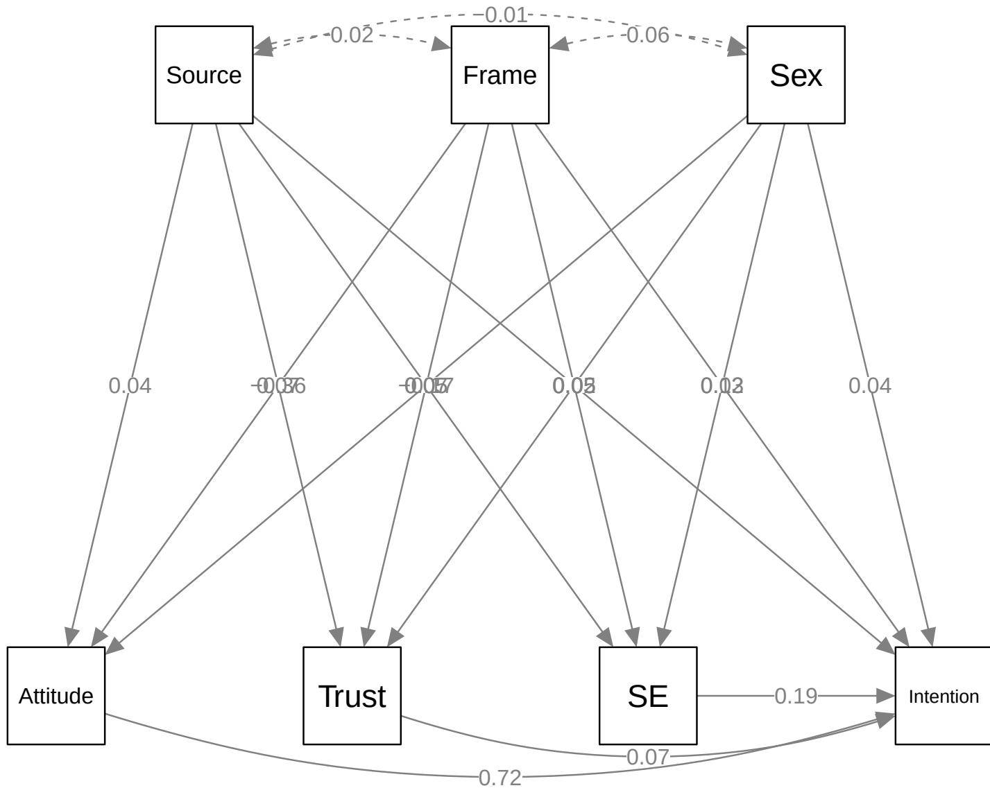
Mediation Model (H1-H6)
