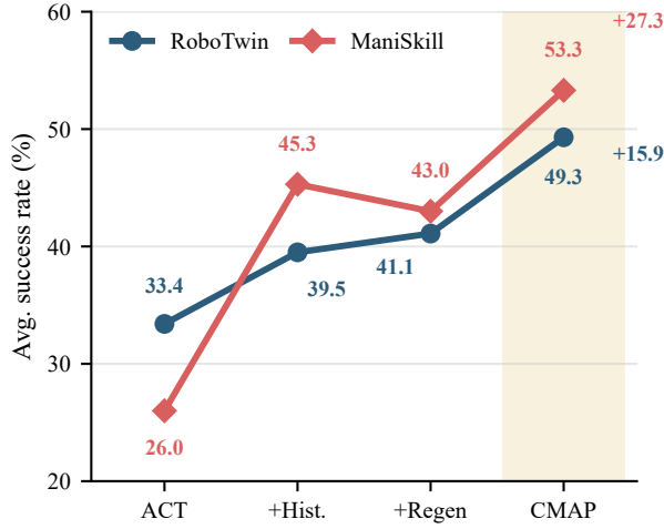
Fig. 3. Component ablations on the fixed RoboTwin diagnostic suite and ManiSkill. +Hist. adds executed-action history, +Regen adds masked span regeneration, and CMAP adds score-guided span selection; labels report macro-averages and CMAP gains over ACT.
