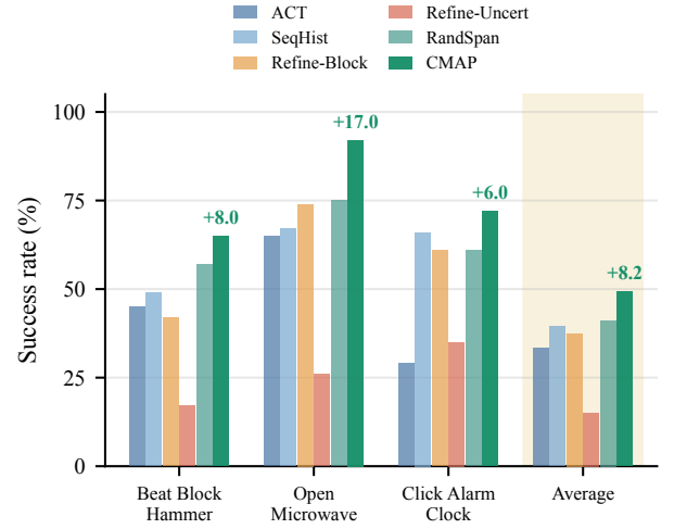
Fig. 4. Task-level ablations on three tasks from the fixed RoboTwin diagnostic suite and its eight-task macro-average. Labels above CMAP show gains over the strongest alternative.
