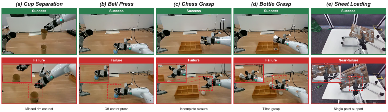
Fig. 8. Real-world execution examples on AGIBOT G1 and Kuavo 4 Pro. Top: success. Bottom: failures for Cup Separation , Bell Press , Chess Grasp , and Bottle Grasp , plus a recovered near-failure for Sheet Loading . Red callouts mark critical contact regions.
