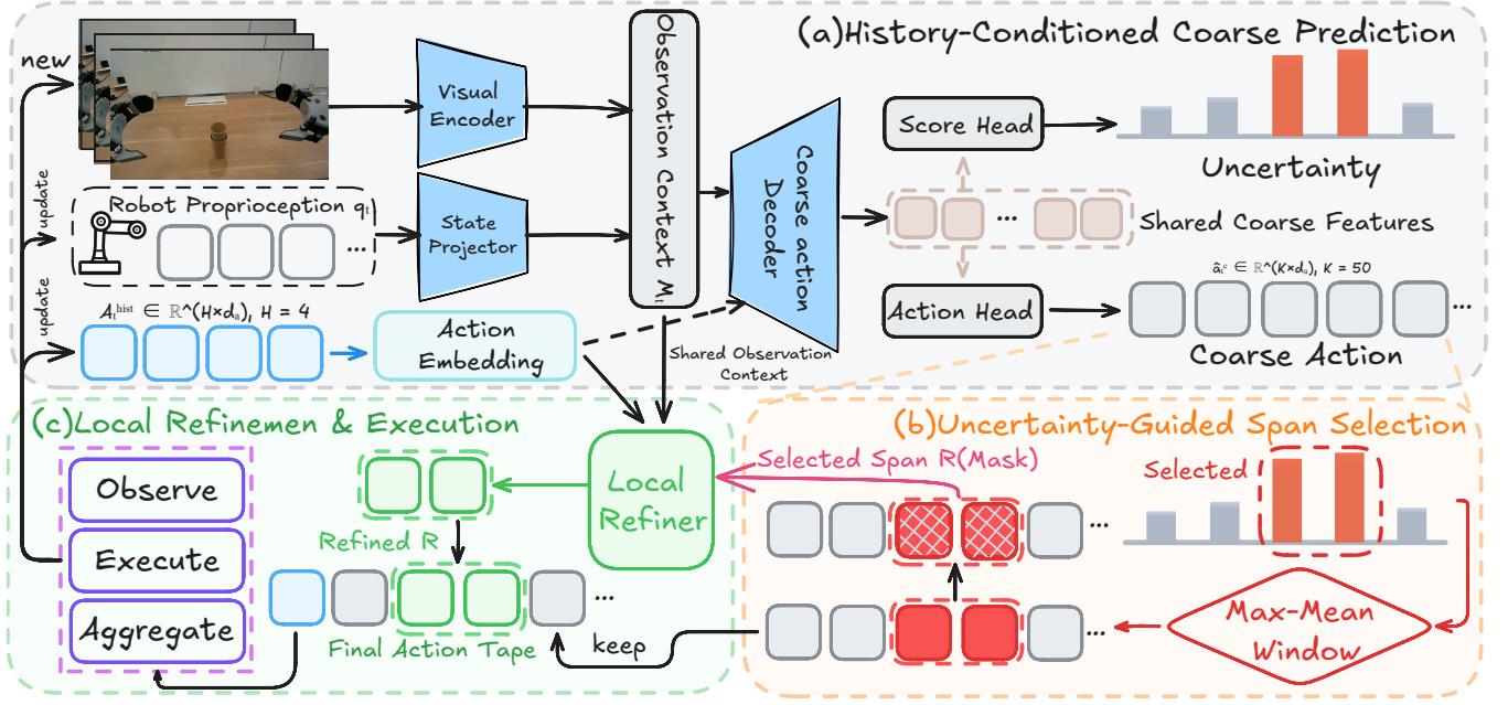
Fig. 2. Overview of CMAP. (A) The current observation and visible executed-action history of length H condition a coarse prediction of K future actions and per-step span-selection scores. (B) Contiguous future windows are ranked by their mean scores, and the highest-scoring window defines the selected span \mathcal{R} . (C) The local refiner regenerates only \mathcal{R} , merges it with the preserved coarse actions, and executes the resulting action tape with receding-horizon control.
