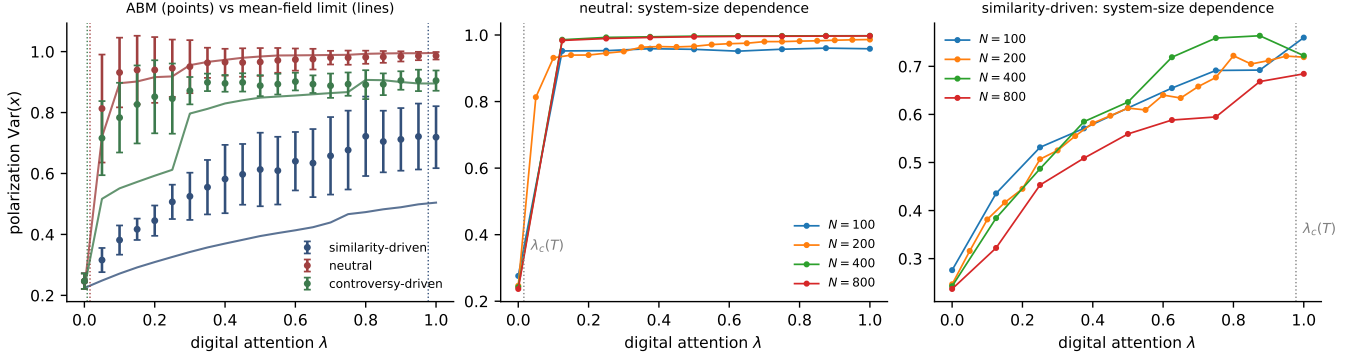
FIG. 9. Radicalization onset in the digital attention share. Left: final polarization versus \lambda for the three platforms; points are the spatial ABM ( N = 200 , 12 seeds), solid lines the McKean–Vlasov mean-field limit of Eq. (12), dotted verticals the parameter-free finite-horizon crossovers \lambda_c(T) of Table I. Centre and right: system-size dependence of the \text{Var}(x) – \lambda curves for the neutral and similarity platforms.
