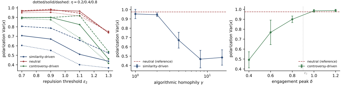
FIG. 7. Robustness of the inversion. Left: final polarization versus the repulsion threshold \epsilon_2 for \eta = 0.2/0.4/0.8 (dotted/solid/dashed); colours denote platforms (blue similarity, red neutral, green controversy). Centre: similarity platform versus algorithmic homophily \gamma , with the neutral platform as reference. Right: controversy platform versus engagement peak \delta ; the dotted line marks \delta = \epsilon_2 . Mean \pm s.d. over 6 runs.
