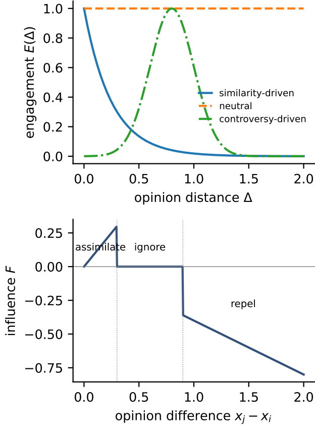
FIG. 5. Level-4 ingredients. Top: the three engagement kernels of Eq. (7) ( \gamma = 4 , \delta = 0.8 , s = 0.2 ). Bottom: the assimilation-indifference-repulsion influence function of Eq. (4) ( \epsilon_1 = 0.3 , \epsilon_2 = 0.9 , \eta = 0.4 ).
