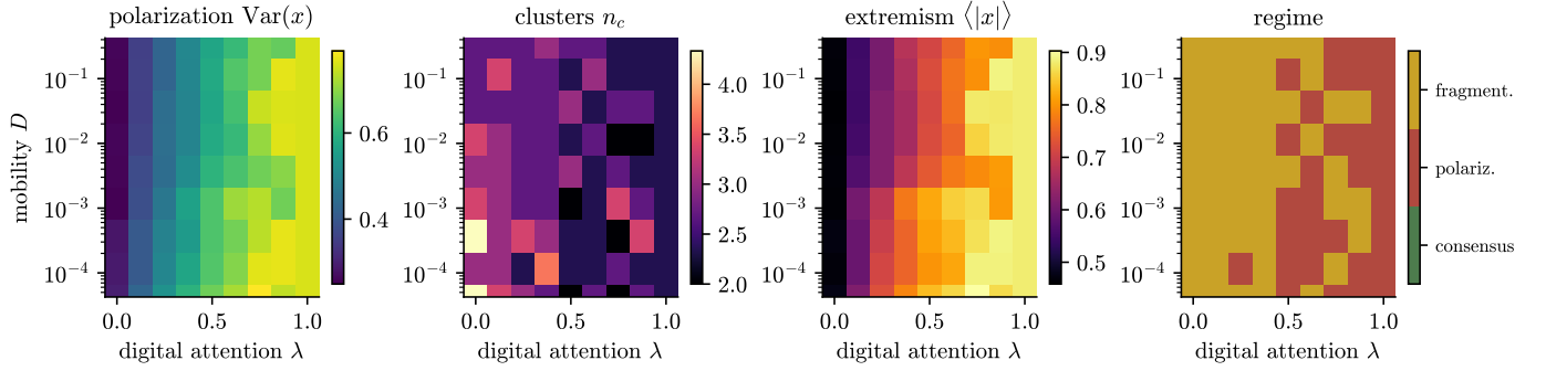
Figure 10: Phase diagram of the full Level-4 model (similarity-driven engagement, repulsion, heavy-tailed influence) in the mobility–digital-attention plane. From left to right: polarization \text{Var}(x) , cluster count n_c , extremism \langle |x| \rangle , and the majority categorical state over 3 realisations per grid point. The panel is a coarse regime map intended to reveal qualitative structure; at 3 realisations per point the boundaries between regimes are not sharply resolved. At \lambda = 1 the physical layer is off and the dynamics is independent of D by construction.
