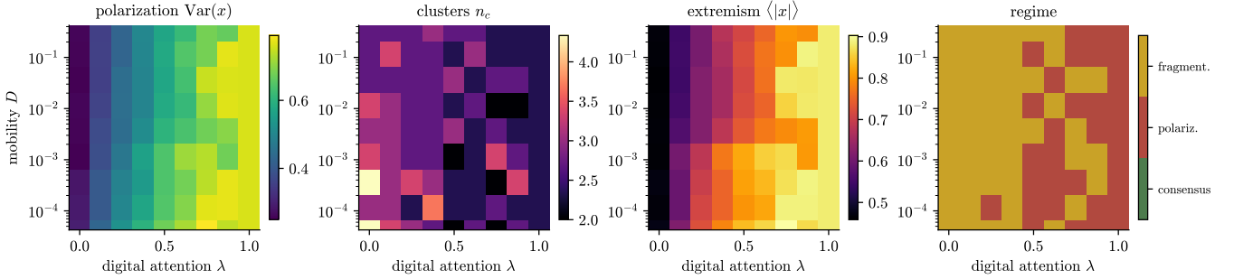
FIG. 10. Phase diagram of the full Level-4 model (similarity-driven engagement, repulsion, heavy-tailed influence) in the mobility–digital-attention plane. From left to right: polarization \text{Var}(x) , cluster count n_c , extremism \langle |x| \rangle , and the majority categorical state over 3 realisations per grid point. The panel is a coarse regime map intended to reveal qualitative structure; at 3 realisations per point the boundaries between regimes are not sharply resolved. At \lambda = 1 the physical layer is off and the dynamics is independent of D by construction.
