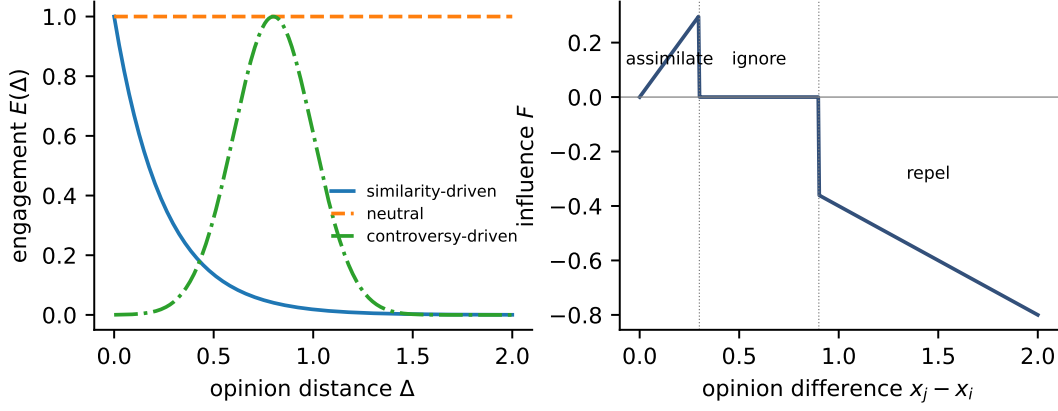
FIG. 5. Level-4 ingredients. Left: the three engagement kernels of Eq. (7) ( \gamma = 4 , \delta = 0.8 , s = 0.2 ). Right: the assimilation–indifference–repulsion influence function of Eq. (4) ( \epsilon_1 = 0.3 , \epsilon_2 = 0.9 , \eta = 0.4 ).
