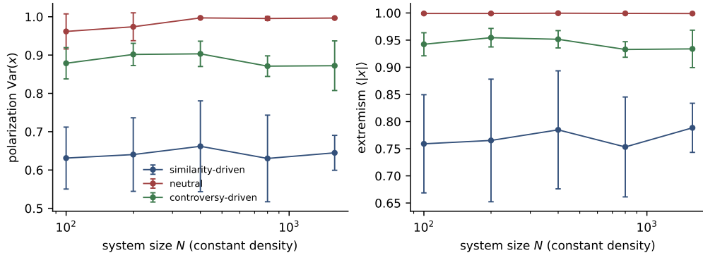
FIG. 8. System-size dependence of the inversion at constant density ( L = \sqrt{N/200} ), \lambda = 0.6 . Polarization (left) and extremism (right) for the three platforms, N = 100 –1600.
