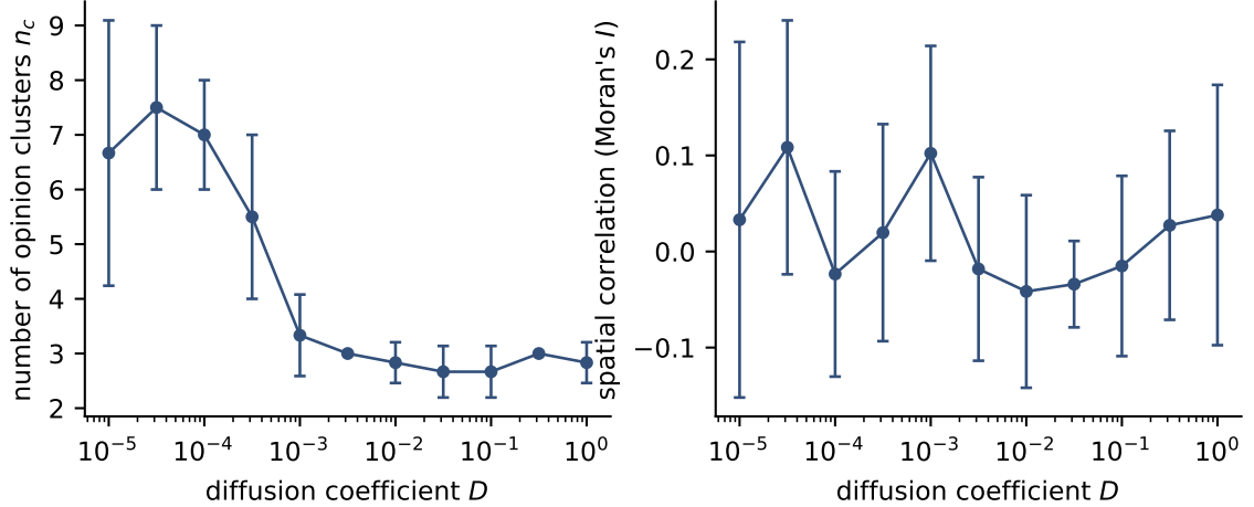
FIG. 2. Level-1 sweep over the diffusion coefficient. Left: mean number of surviving opinion clusters. Right: Moran's I between opinion and position (mean \pm s.d. over 6 realisations). Mobility interpolates between local fragmentation and mean-field behaviour while the spatial-opinion correlation stays at noise level throughout.
