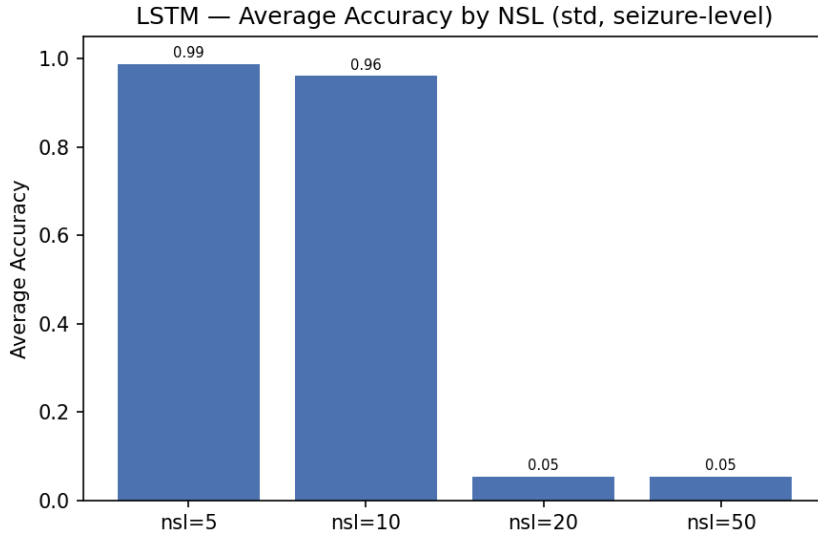
Figure 10: Average accuracy for LSTM-std with varying non-seizure episode lengths.
