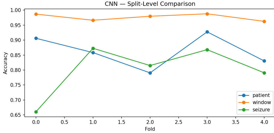
Figure 11: CNN accuracy per fold under patient, window, and seizure-level splits.
