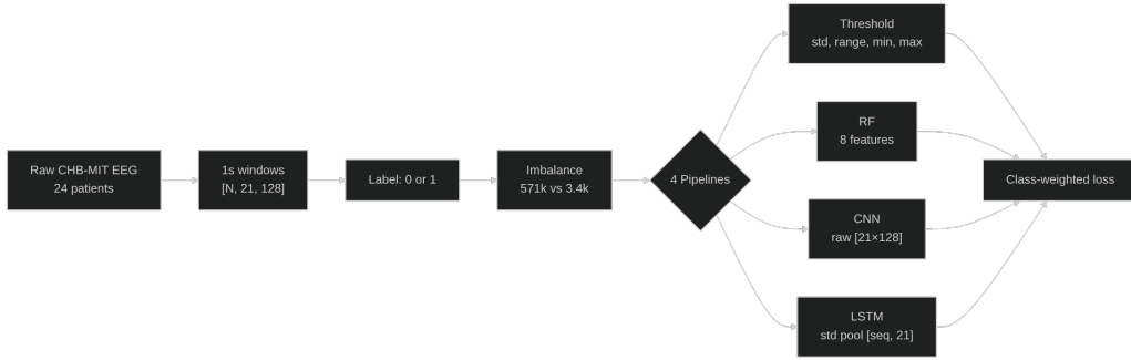
Figure 3: Data preprocessing and pipeline branching. All four pipelines start from the same raw EEG windows; class weighting (not shown) compensates for the severe class imbalance.
