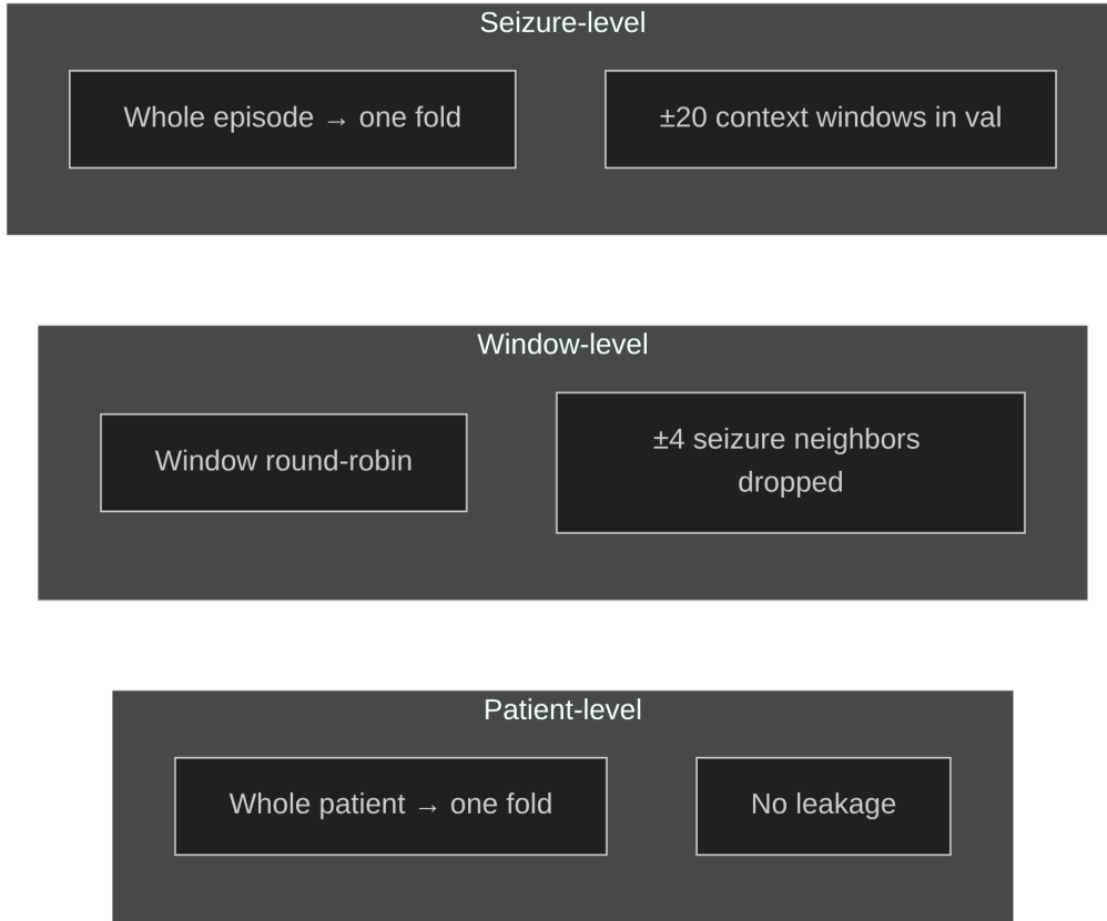
Figure 4: Cross-validation strategies: patient-level (threshold, RF, CNN), window-level (CNN alternative), and seizure-level (LSTM).
