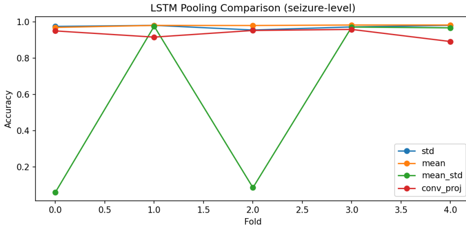
Figure 8: Per-fold accuracy for LSTM pooling options evaluated under seizure-level CV.
