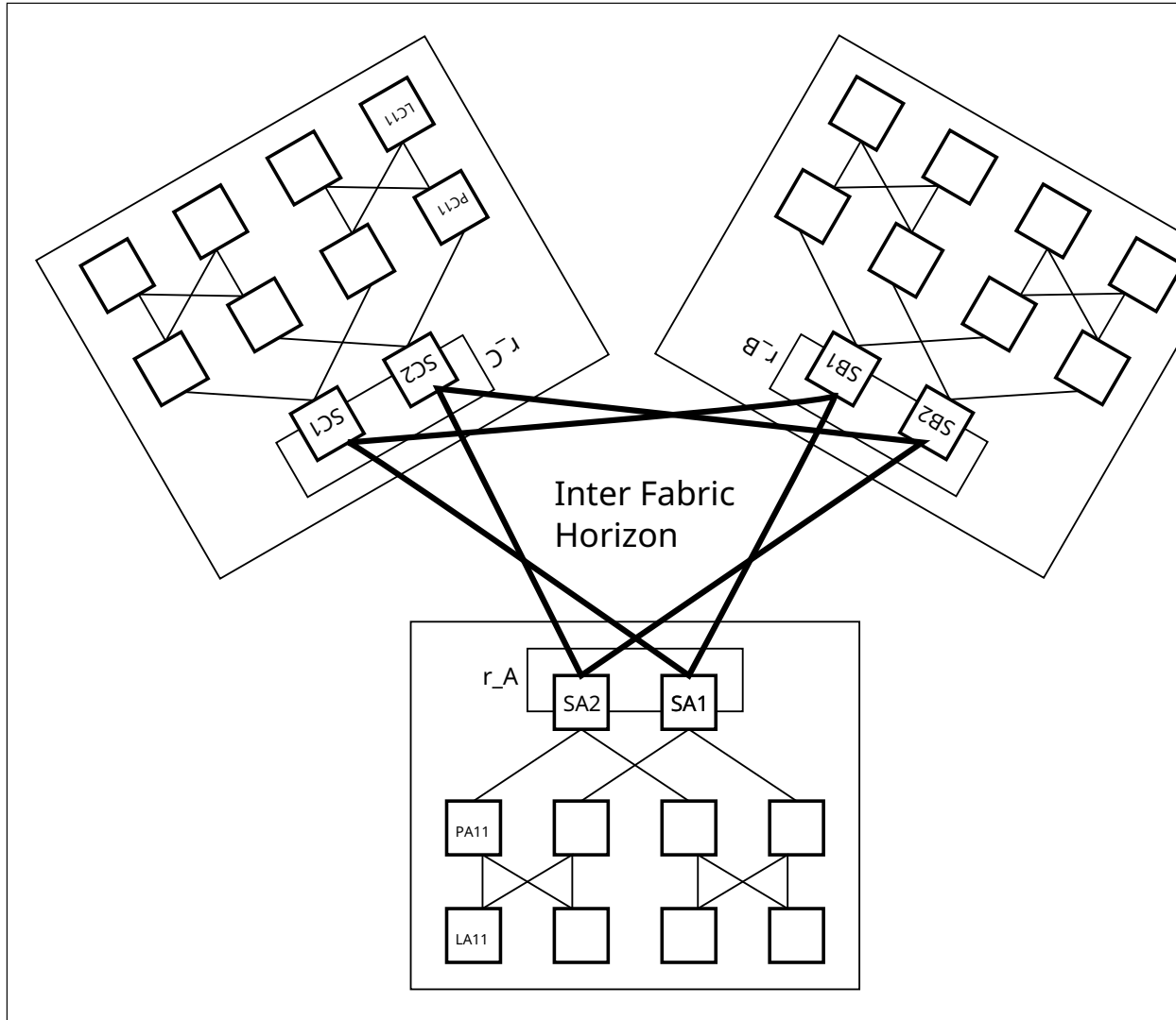
Figure 4: Multi-Plane CLOS Fabrics Connected in Sparse Dragonfly
