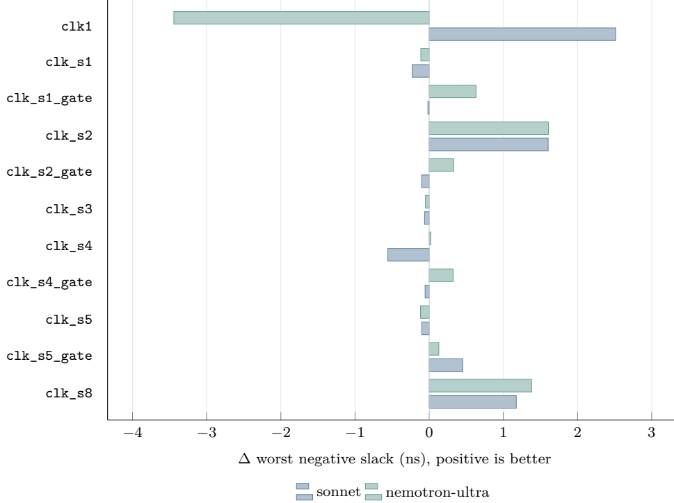
Figure 4: Slack change per clock domain, both routed variants against the same baseline. The two bars agree closely only where the edit did the work.
