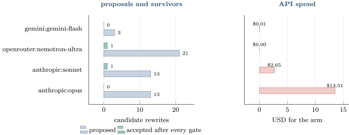
Figure 6: Four models, one invocation, the same three targets and the same gates. Spend and survival are not related the way the price list suggests.
