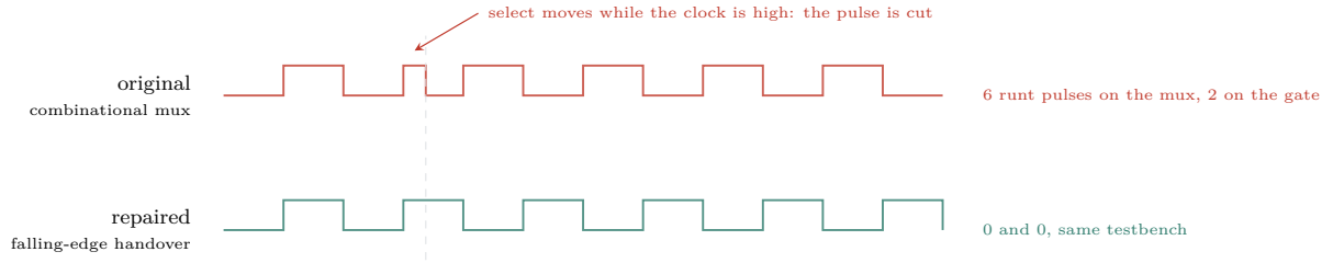
Figure 2: The clock-divider mux before and after the repair, with the pulse widths a simulation measured on each. The traces are schematic; the counts beside them are the testbench’s, and the upper row is the original RTL run through the identical stimulus.
