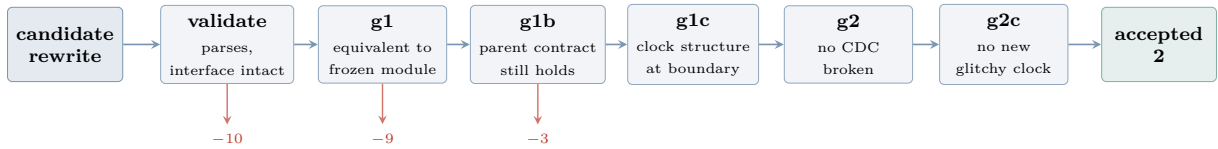
Figure 3: Every gate a rewrite must pass, with the number of candidates each one rejected across all four models. A gate rejects on its own evidence and reports what it found; the model’s next attempt answers that, rather than being asked the same question again.
