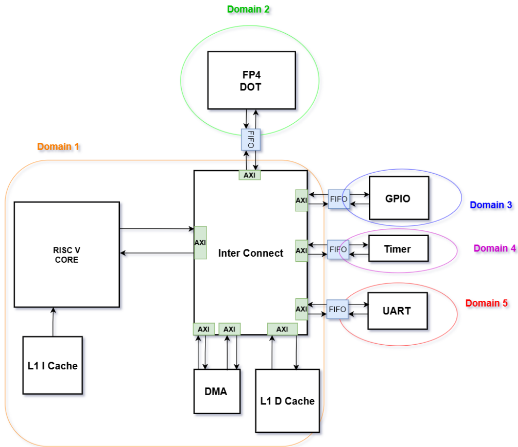
Figure 3: Nebula SoC benchmark: five asynchronous clock domains, each peripheral crossing into the AXI interconnect through a dedicated async FIFO.
