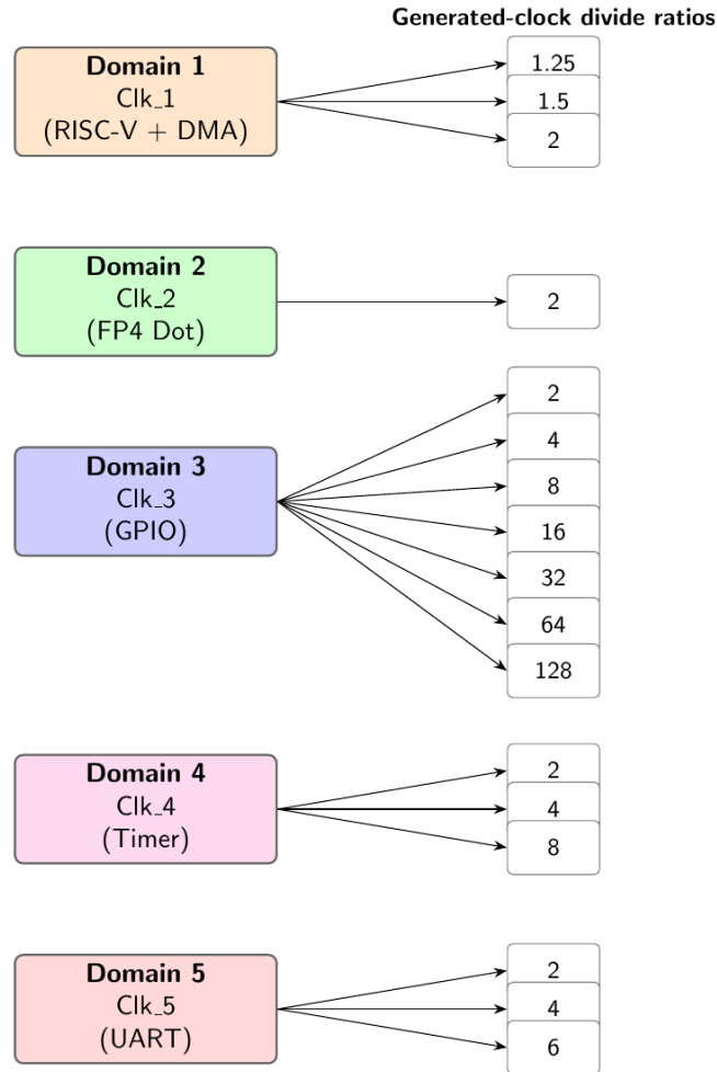
Figure 4: Generated-clock divide ratios per domain — 1.25/1.5/2 on domain 1, 2 on domain 2, seven octave steps (2 through 128) on domain 3, 2/4/8 on domain 4, 2/4/6 on domain 5.
