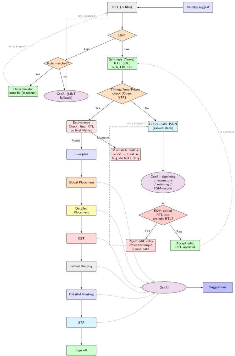
Figure 2: Closed-loop RTL-fix pipeline. Every GenAI edit is checked against pre-edit RTL before acceptance; the final equivalence check gates entry to floorplanning, and a mismatch there halts and reports rather than retrying.
