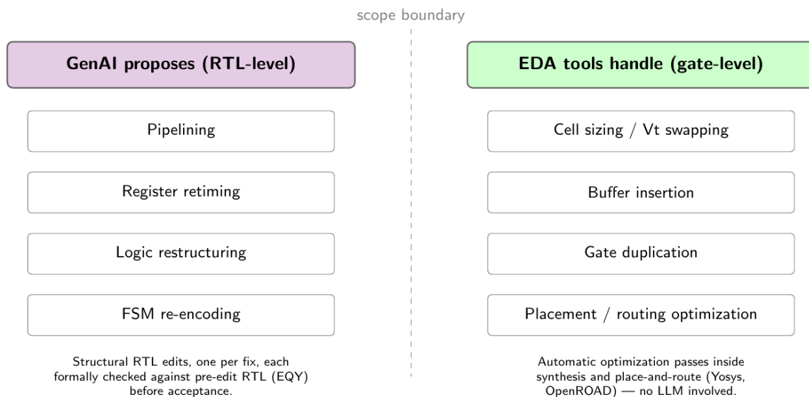
Figure 1: Scope split: GenAI proposes RTL-level structural edits; EDA tools (Yosys/OpenROAD) continue to handle gate-level optimization automatically, as they already do today.
