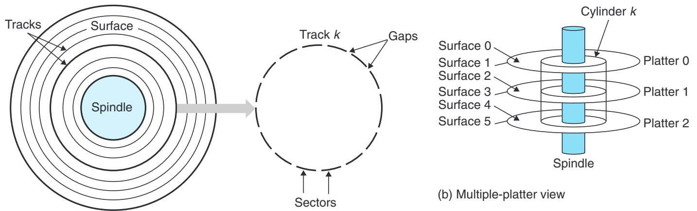
(a) Single-platter view
