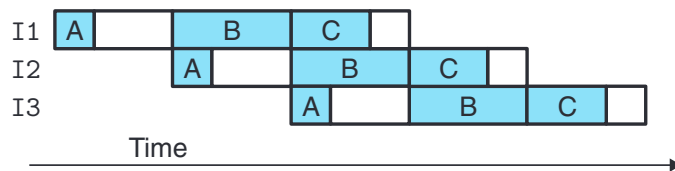
(b) Pipeline diagram
