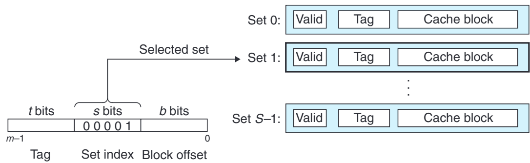
Figure 6.28 Set selection in a direct- mapped cache.
