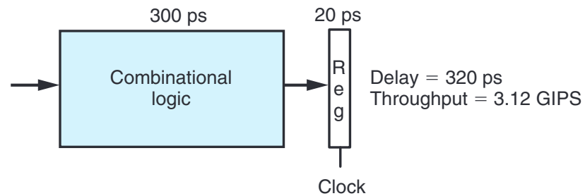
(a) Hardware: Unpipelined
