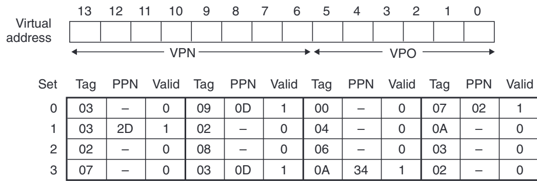
(a) TLB: 4 sets, 16 entries, 4-way set associative
