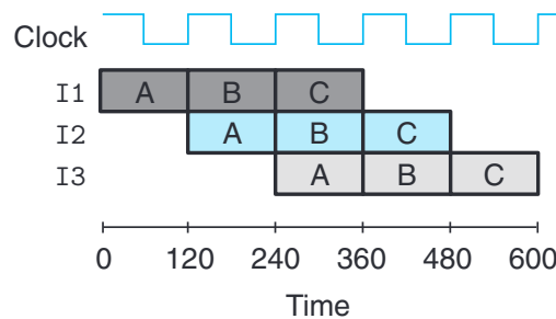
Figure 4.34 Three-stage pipeline timing. The rising edge of the clock signal controls the movement of instructions from one pipeline stage to the next.
