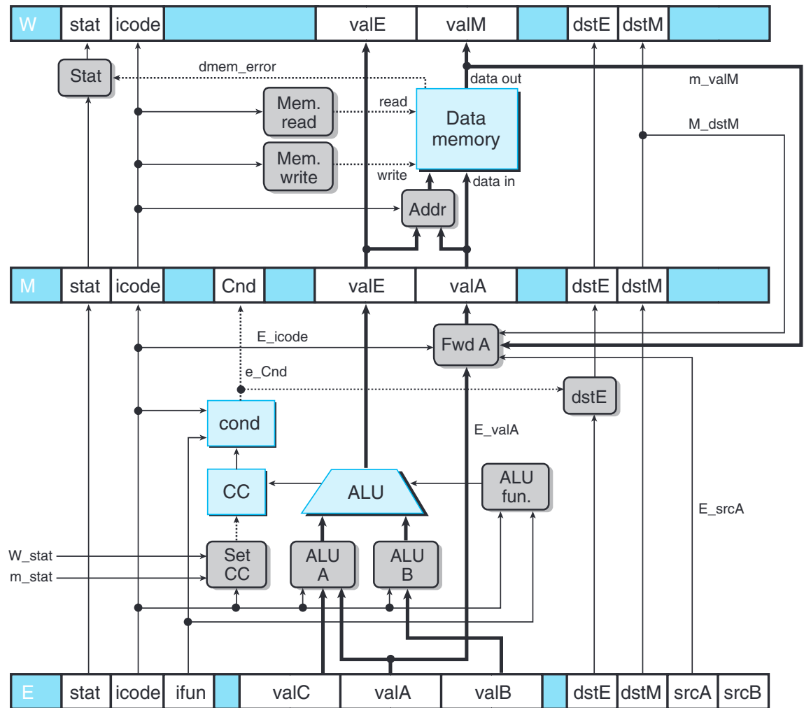
Figure 4.70 Execute and memory stages capable of load forwarding. By adding a bypass path from the memory output to the source of valA in pipeline register M, we can use forwarding rather than stalling for one form of load/use hazard. This is the subject of Problem 4.57.
