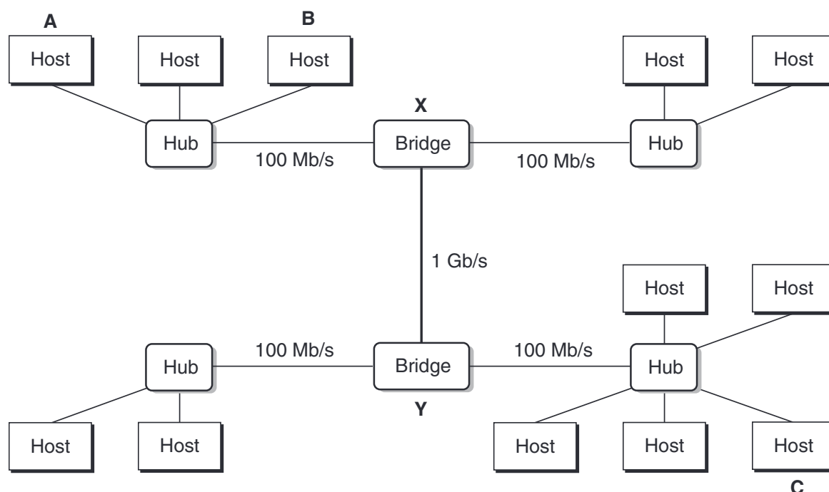
Figure 11.4 Bridged Ethernet segments.
