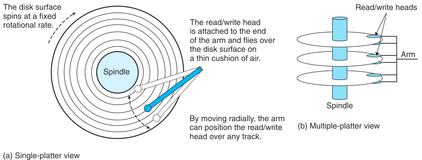
Figure 6.10 Disk dynamics.
