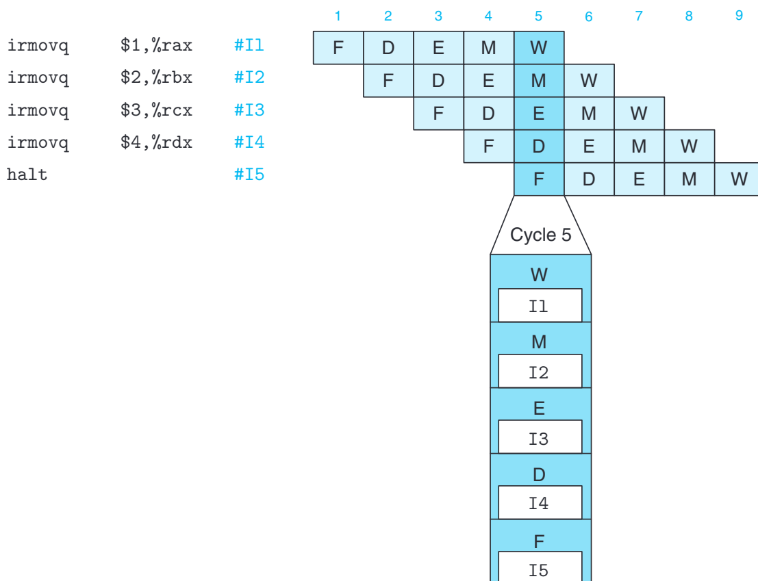
Figure 4.42 Example of instruction flow through pipeline.
