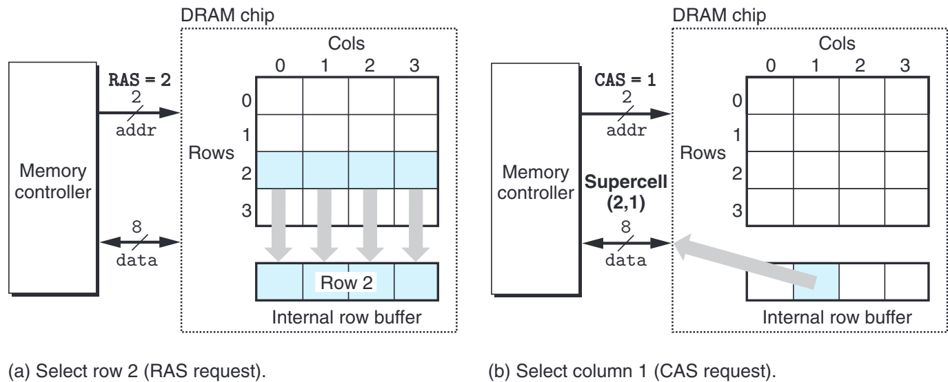
Figure 6.4 Reading the contents of a DRAM supercell.
