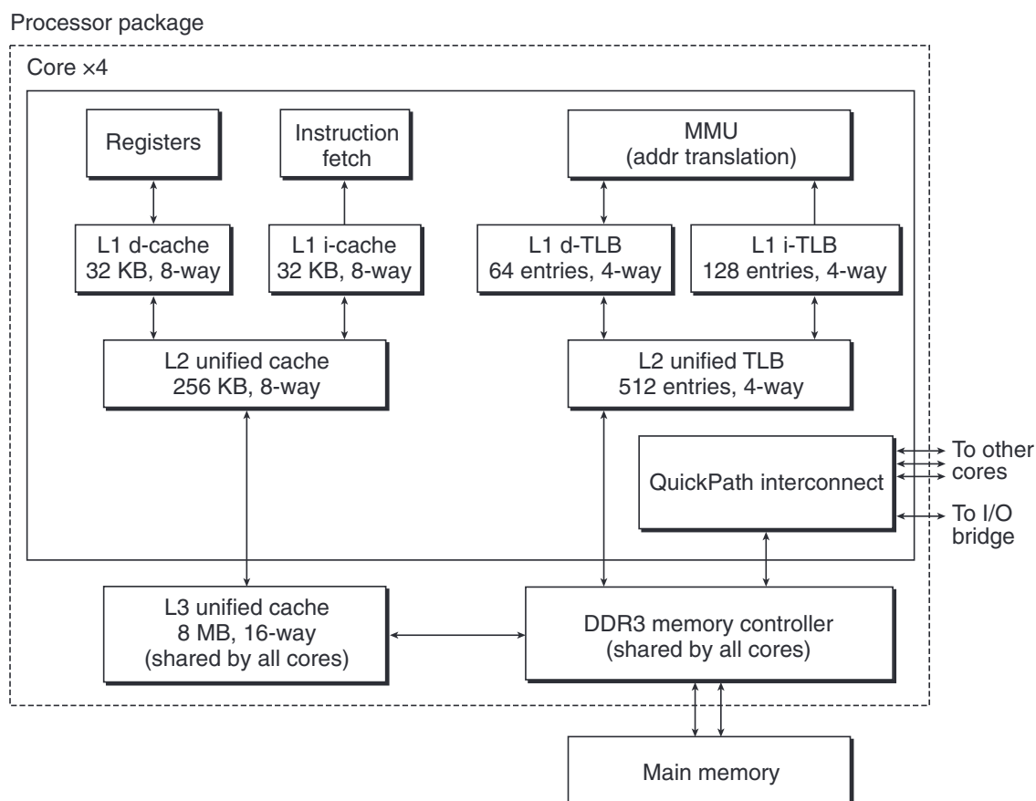
Figure 9.21 The Core i7 memory system.
