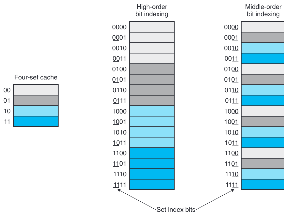
Figure 6.31 Why caches index with the middle bits.
