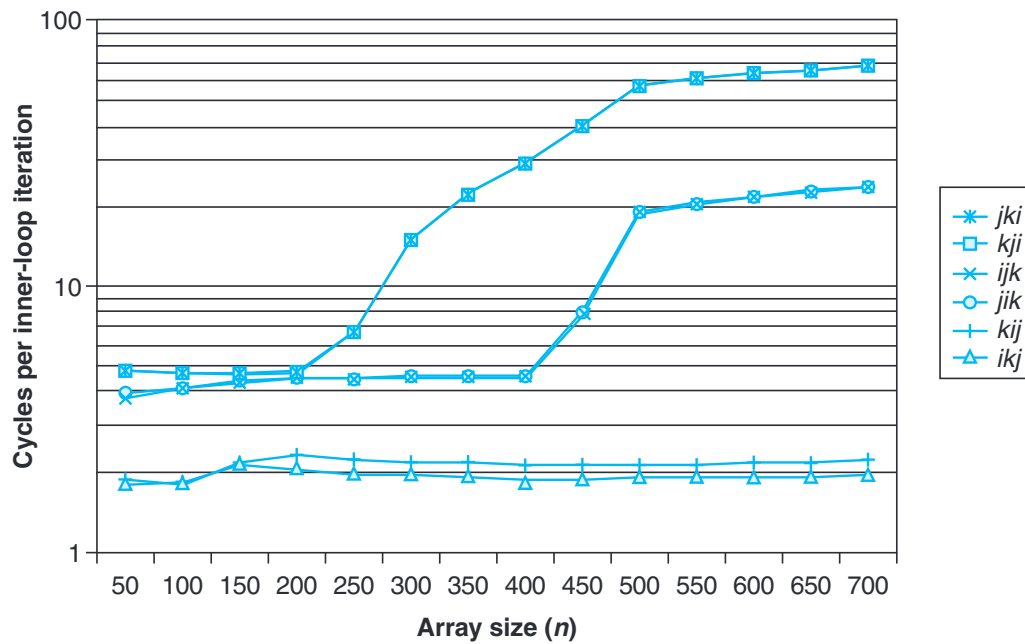
Figure 6.46 Core i7 matrix multiply performance.
