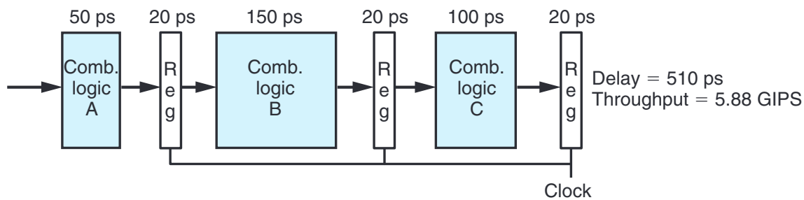
(a) Hardware: Three-stage pipeline, nonuniform stage delays
