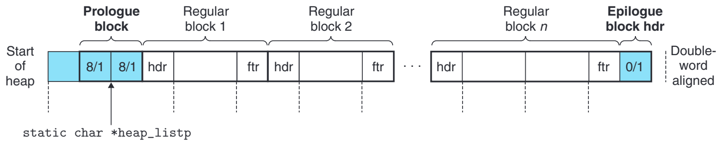
Figure 9.42 Invariant form of the implicit free list.
