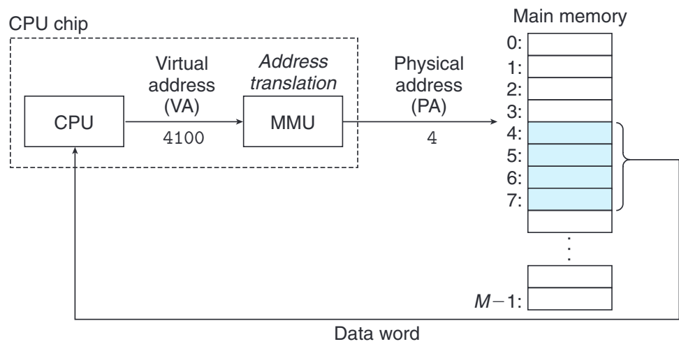
Figure 9.2 A system that uses virtual addressing.
