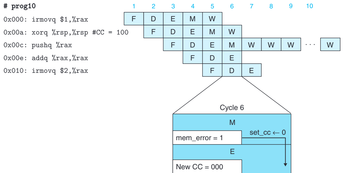
Figure 4.63 Processing invalid memory reference exception. On cycle 6, the invalid memory reference by the pushq %rax instruction causes the updating of the condition codes to be disabled. The pipeline starts injecting bubbles into the memory stage and stalling the excepting instruction in the write-back stage.
