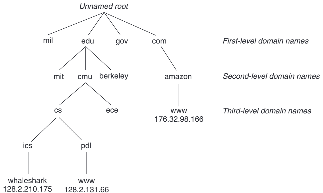
Figure 11.10 Subset of the Internet domain name hierarchy.
