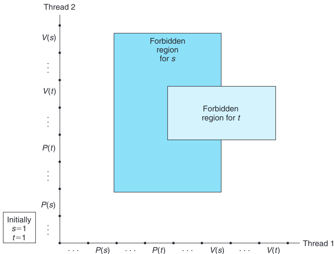
Figure 12.45 Progress graph for a deadlock-free program.
