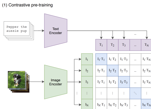
Figure 1: CLIP framework, Source: [5]
