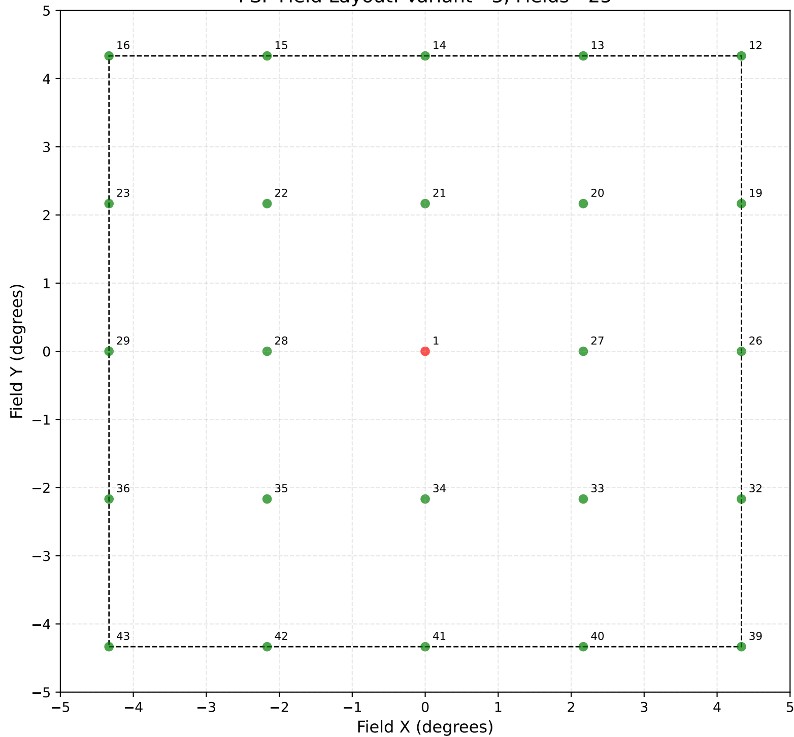
PSF Field Layout: Variant - 3, Fields - 25
