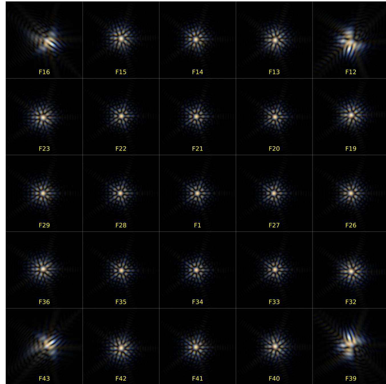
Spatially Arranged PSF Sensor Map Mosaic: 5 x 5 grid, Variant: 3, Fields: 25
