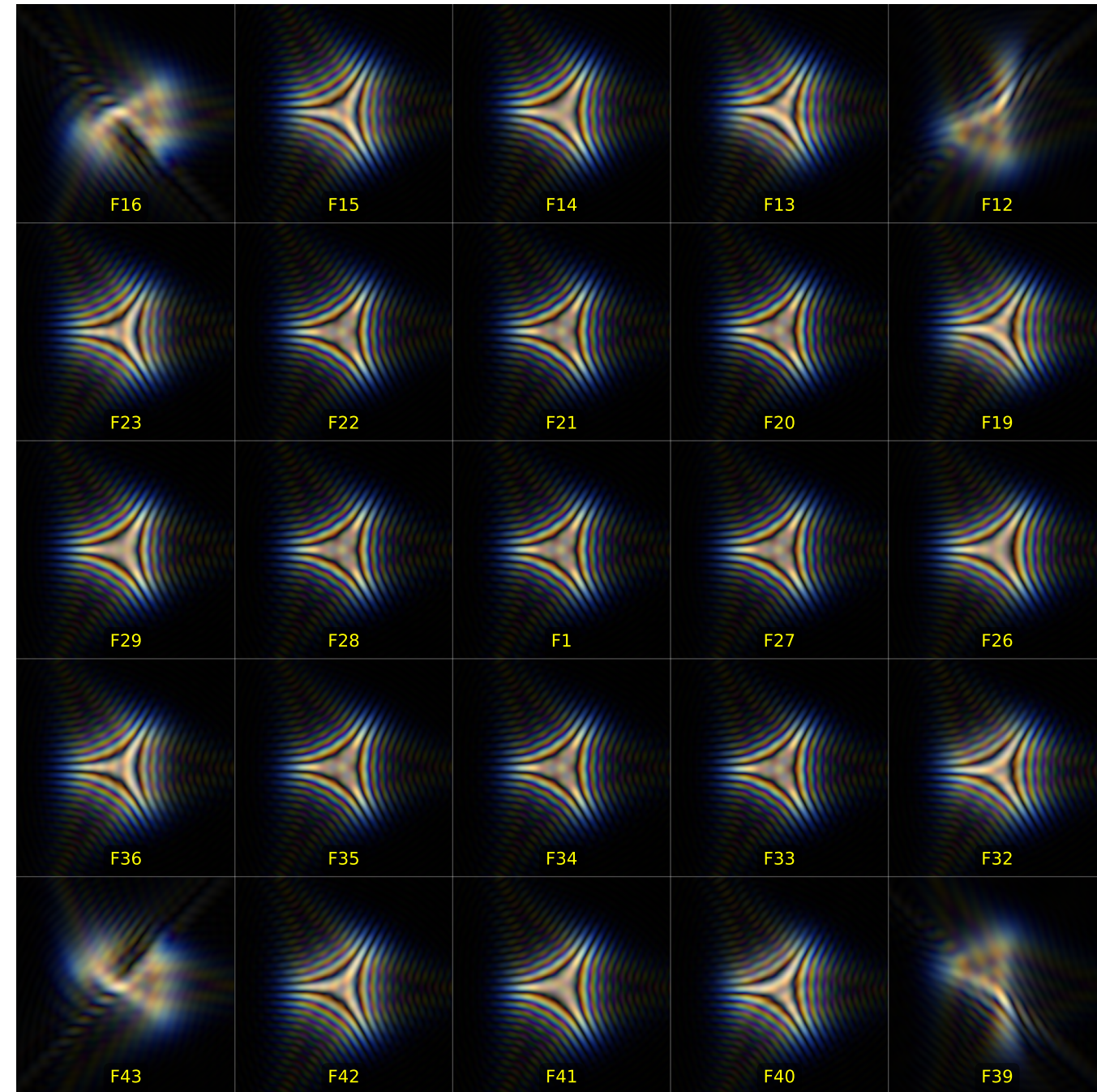
Spatially Arranged PSF Sensor Map Mosaic: 5 x 5 grid, Variant: 2, Fields: 25
