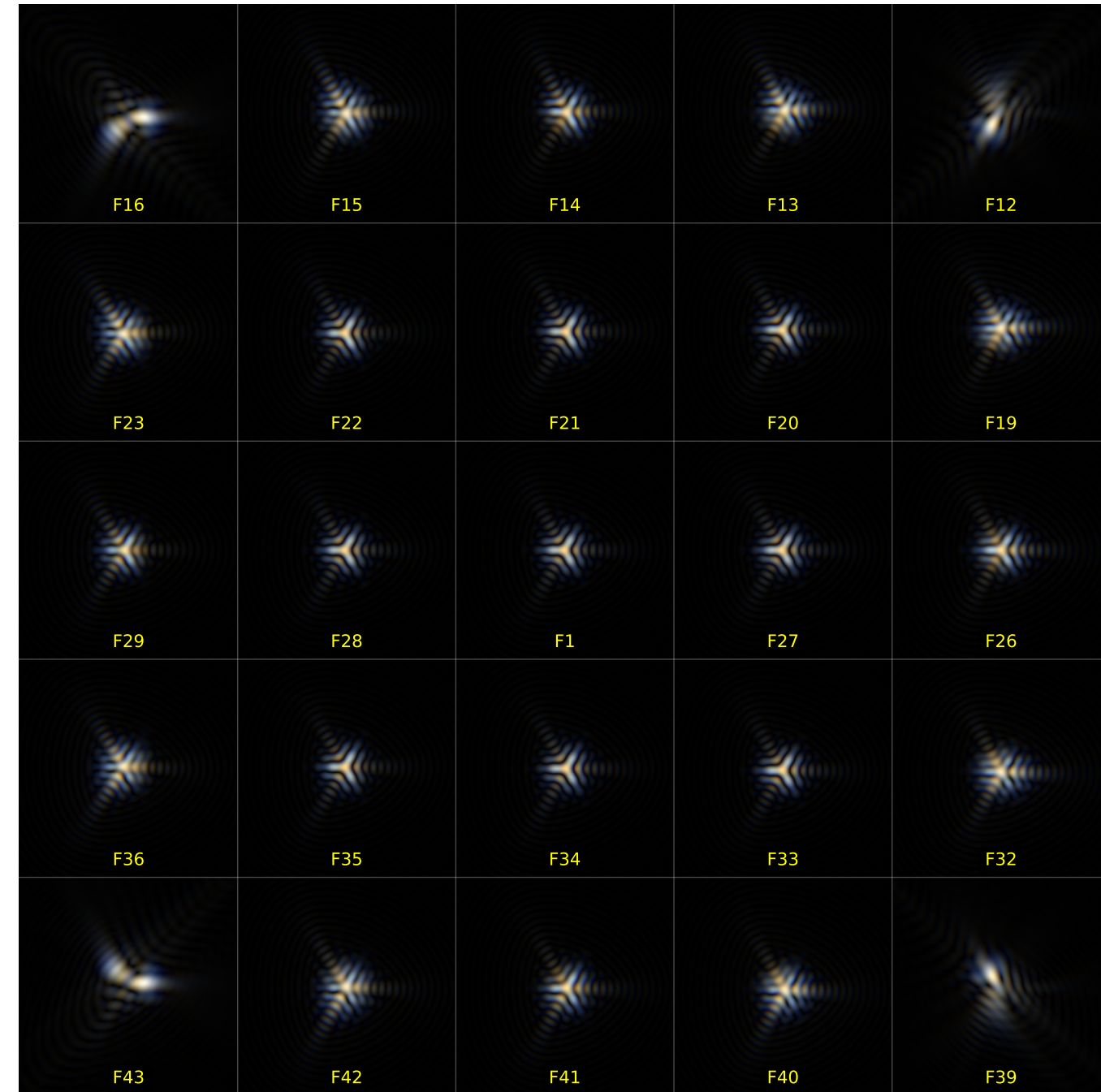
Spatially Arranged PSF Sensor Map Mosaic: 5 x 5 grid, Variant: 1, Fields: 25
