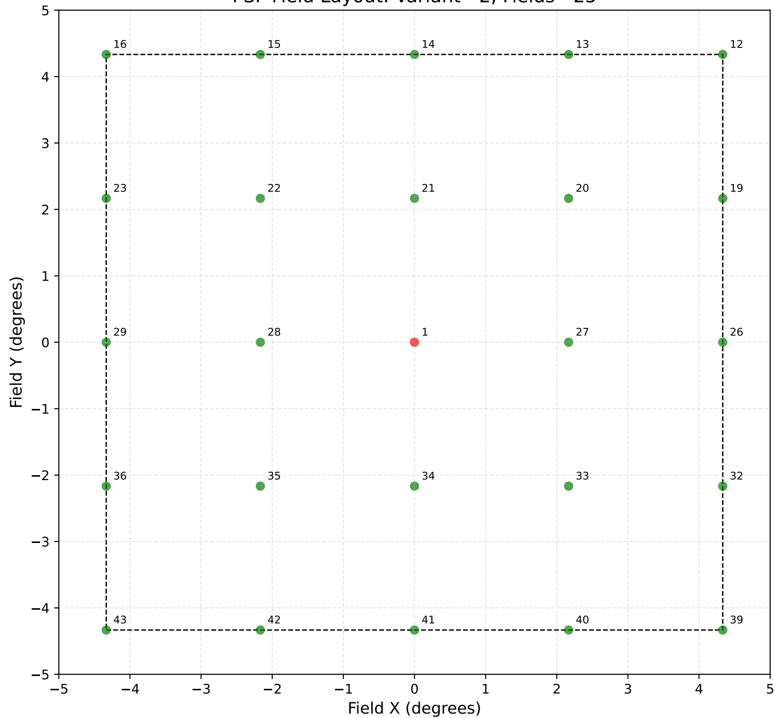
PSF Field Layout: Variant - 2, Fields - 25
