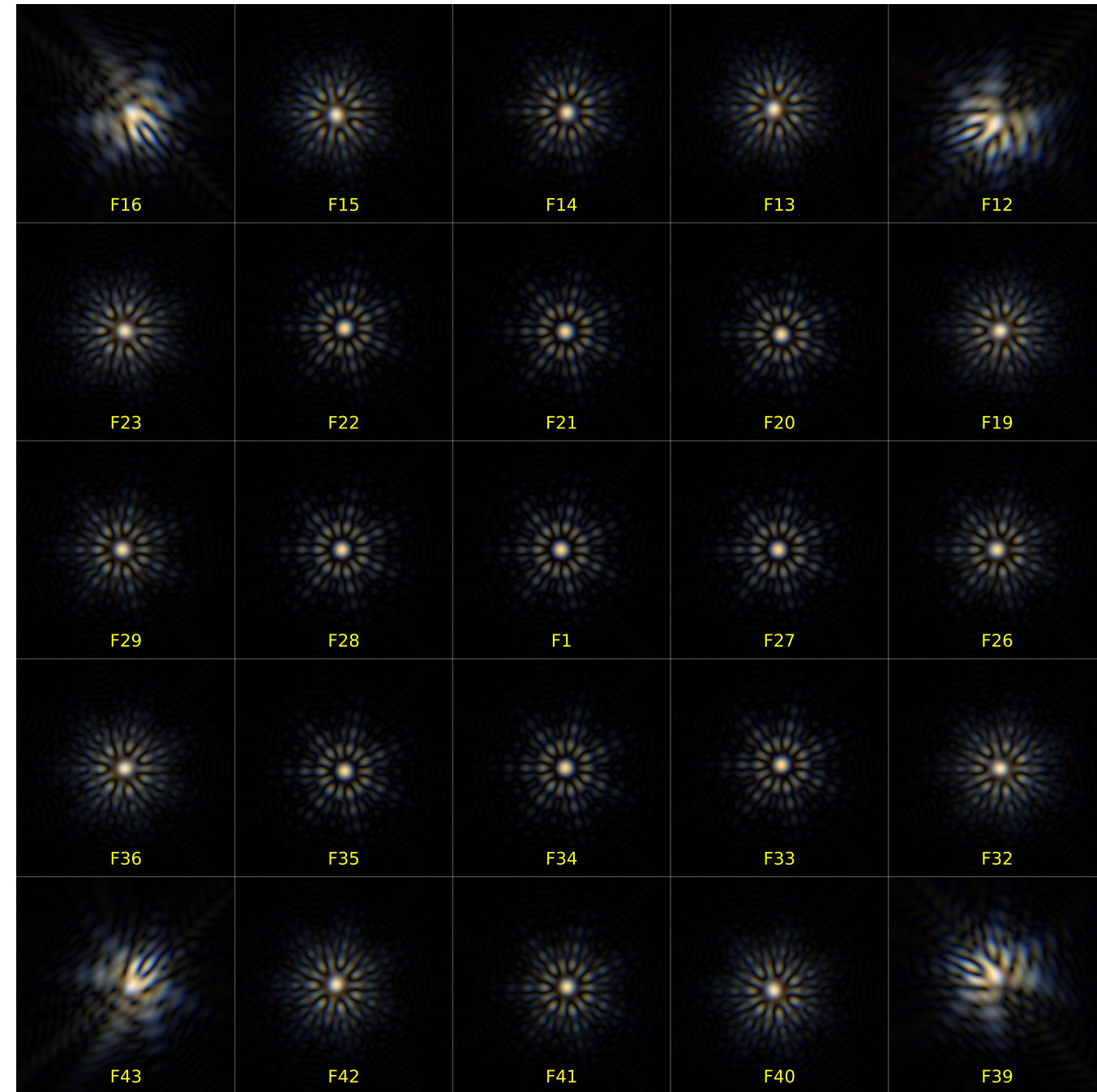
Spatially Arranged PSF Sensor Map Mosaic: 5 x 5 grid, Variant: 5, Fields: 25
