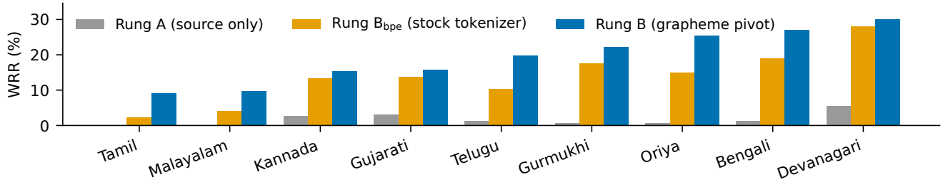
Figure 2. Transfer by script, ordered by Rung B. Source-only baselines (grey) sit at the floor; the grapheme pivot (blue) lifts all nine, and the stock BPE tokenizer (orange) recovers less on every one under identical data, seed and recipe (Sec. 4.3).
