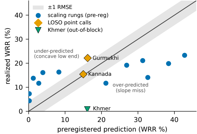
Figure 4. Prospective scorecard: preregistered prediction vs. realized WRR for every quantitative forecast filed before its run, scored against the rule fixed at filing time (shaded \pm 1 RMSE). The in-block LOSO point calls land on the diagonal; the scaling rungs fall off it both ways — under-predicted at low budget, over-predicted at high. Khmer, the out-of-block call, misses low by -3.66-RMSE. Hits and misses are both shown.
