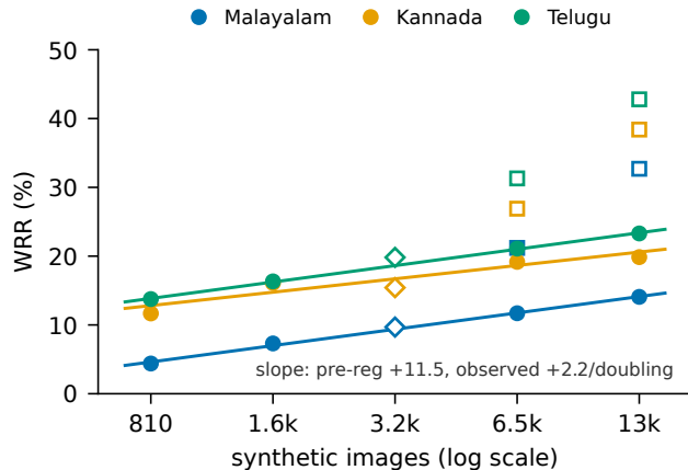
Figure 3. Synthetic-budget dose-response for three held-out scripts. Filled circles: observed WRR on real test images; solid lines: per-script log-linear fits (shared slope +2.235/doubling); open diamonds: the external Rung-B anchor (3240 images); open squares: the preregistered point predictions — their gap above the observed points is the 5.1 \times magnitude miss, reported as filed.
