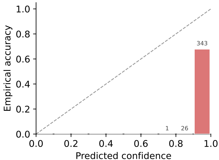
Reliability (fusion) ECE=0.35
