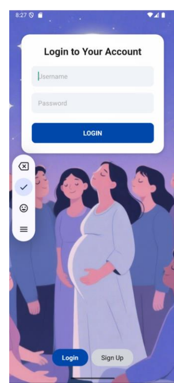
Figure 1. Login screen
