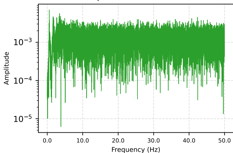
DYN1-10Y — Spectrum
