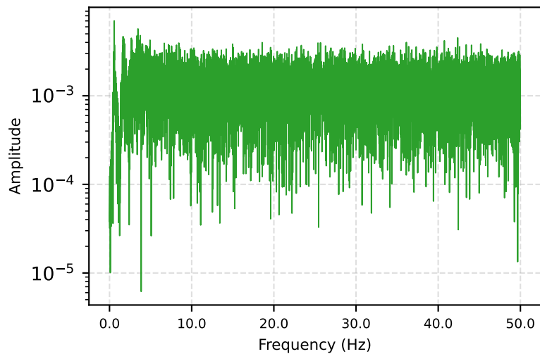
DYN1-20X — Spectrum
