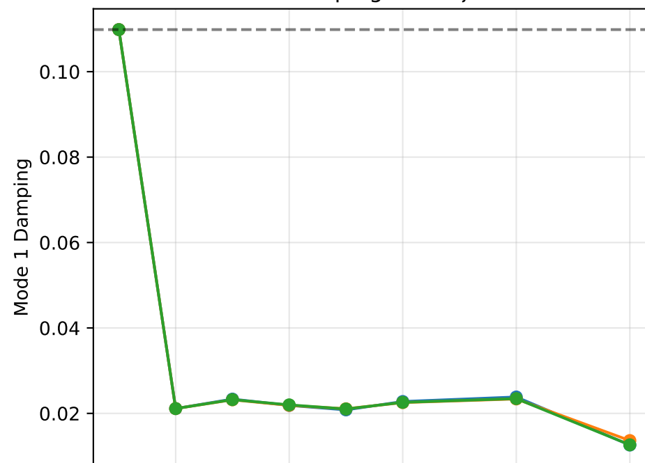
Damping Ratio \zeta
