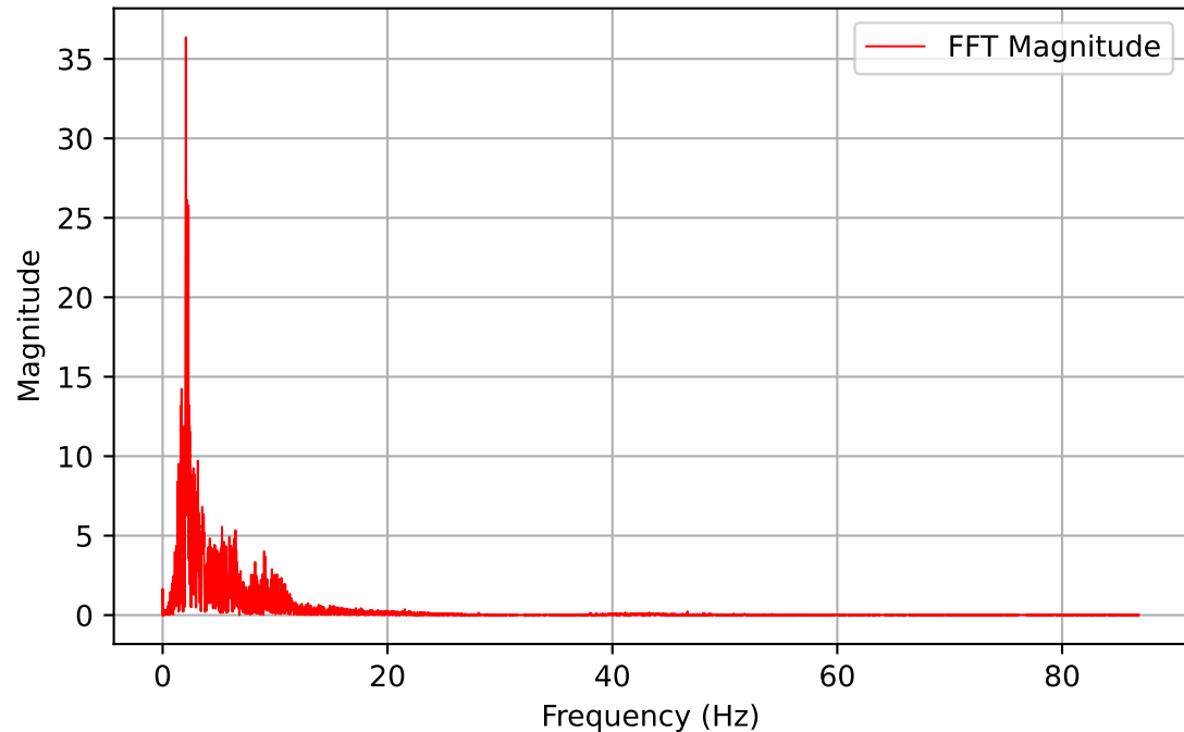
Channel: DYN1-31X (Frequency Domain)
