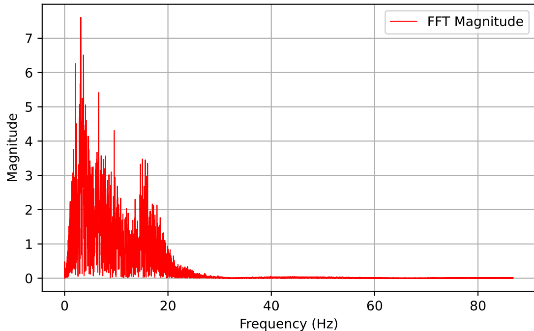
Channel: DYN1-5X (Frequency Domain)
