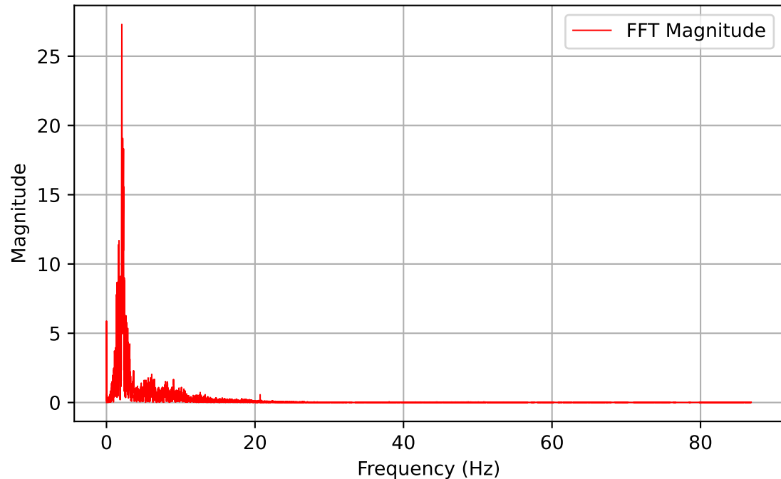
Channel: DYN1-20X (Frequency Domain)
