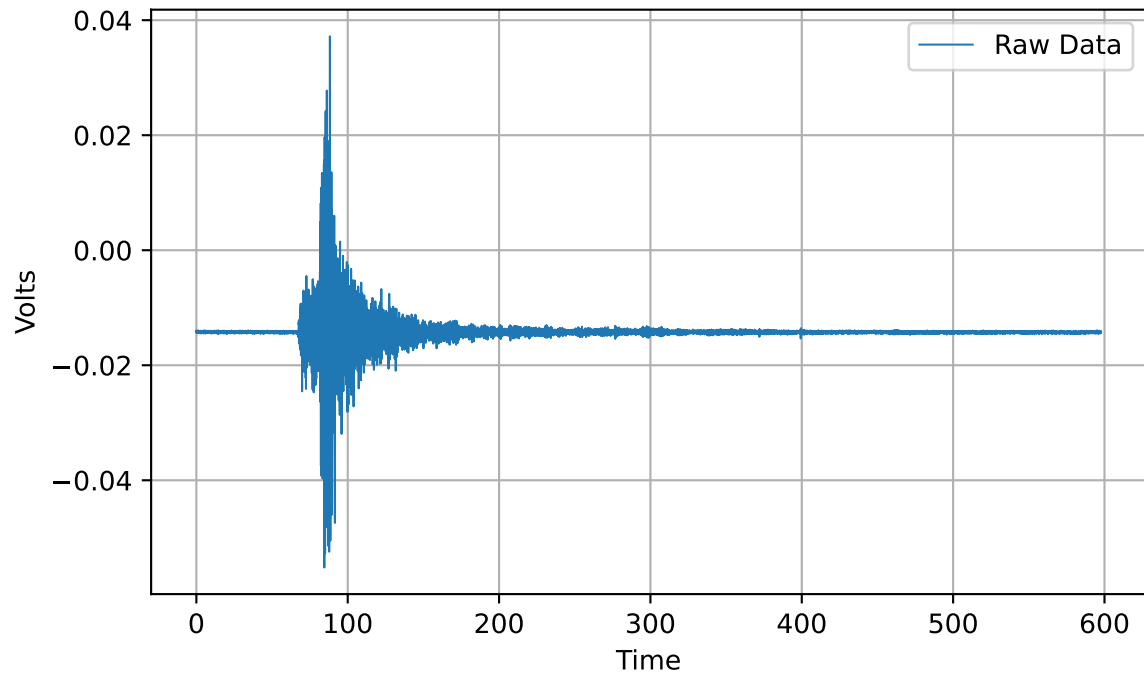
Channel: DYN1-11X (Time Domain)
