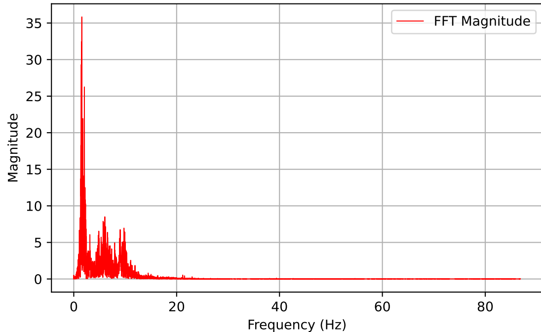
Channel: DYN1-28X (Frequency Domain)
