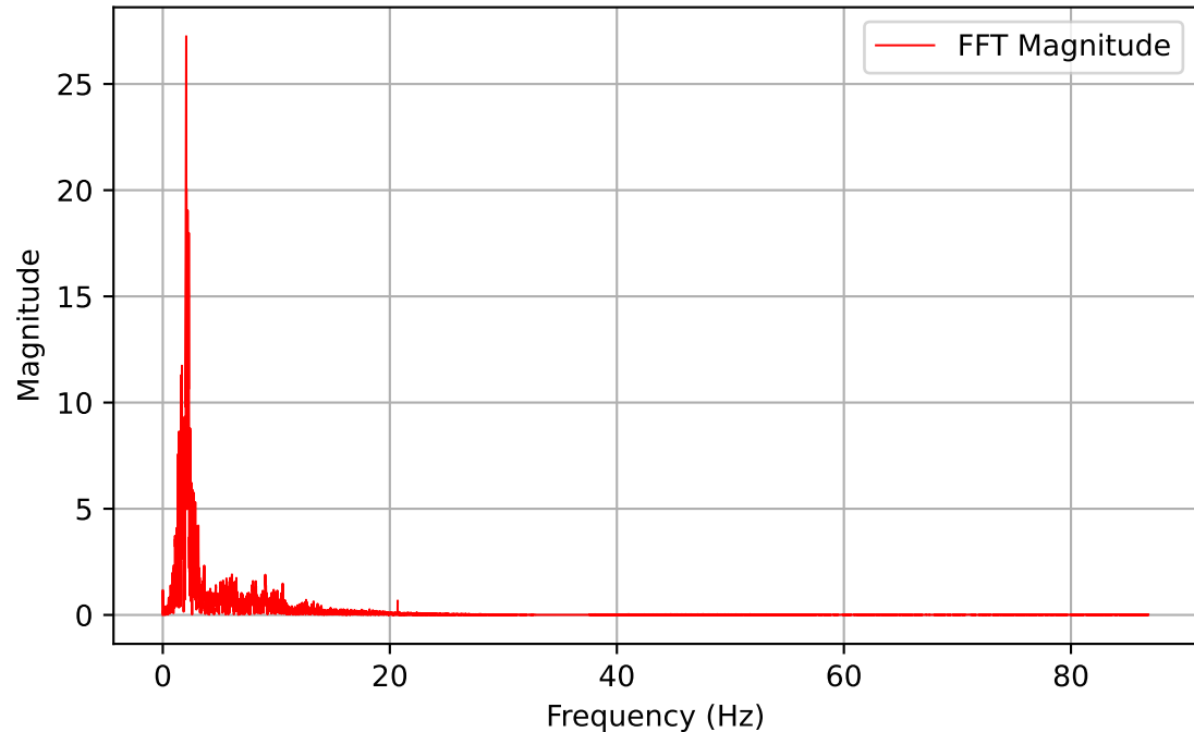
Channel: DYN1-19X (Frequency Domain)
