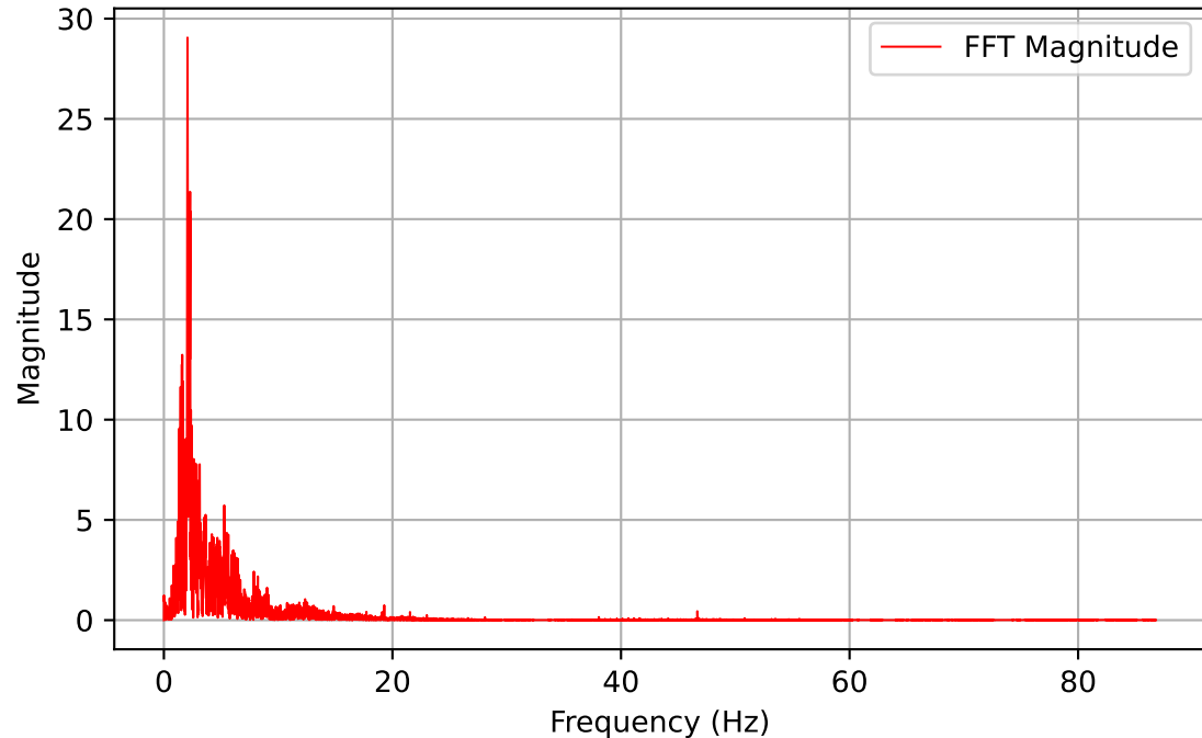
Channel: DYN1-29X (Frequency Domain)
