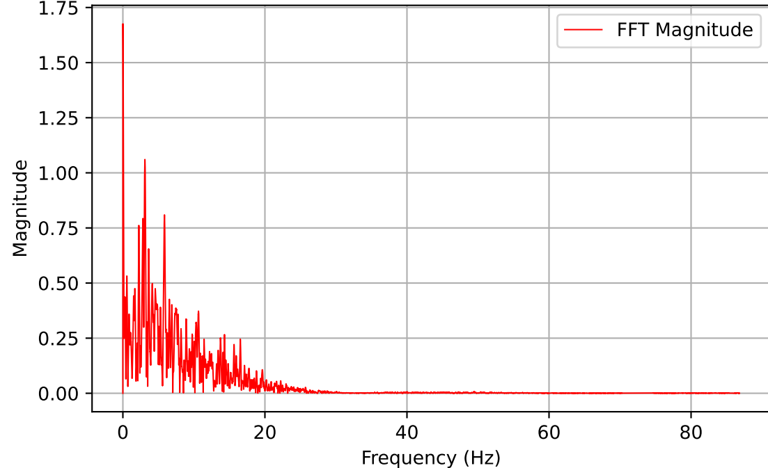
Channel: DYN1-1X (Frequency Domain)
