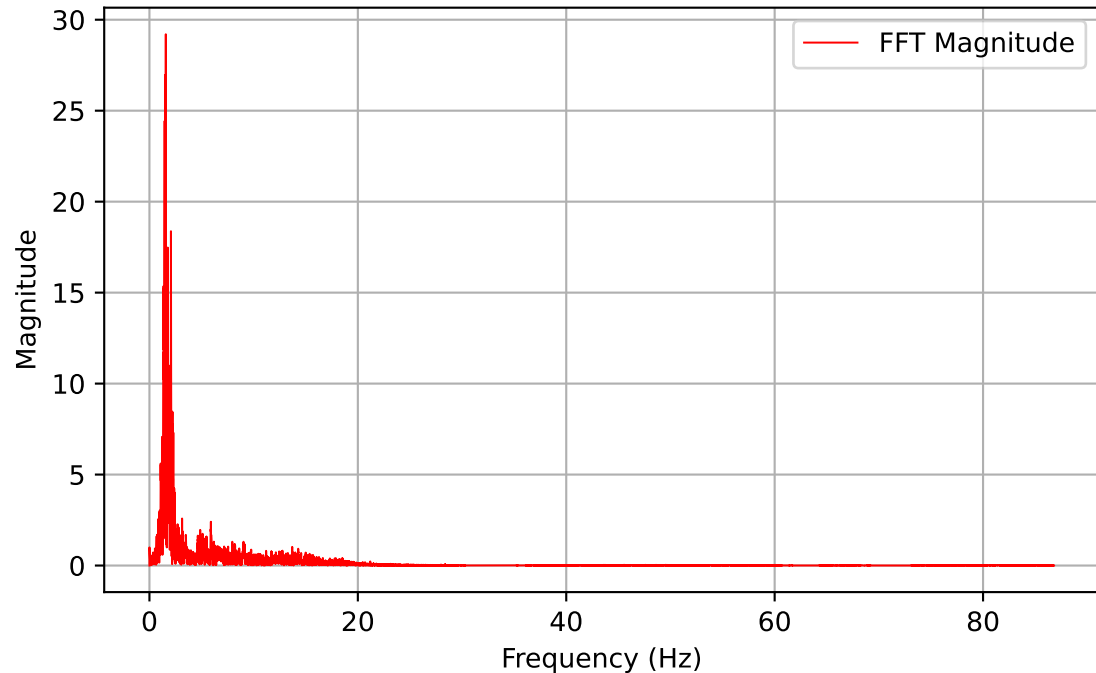
Channel: DYN1-16X (Frequency Domain)
