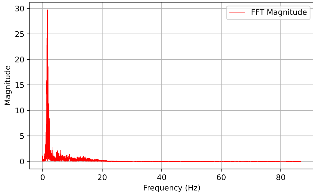
Channel: DYN1-14X (Frequency Domain)
