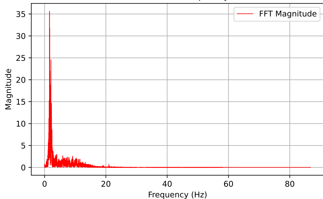
Channel: DYN1-21Y (Frequency Domain)
