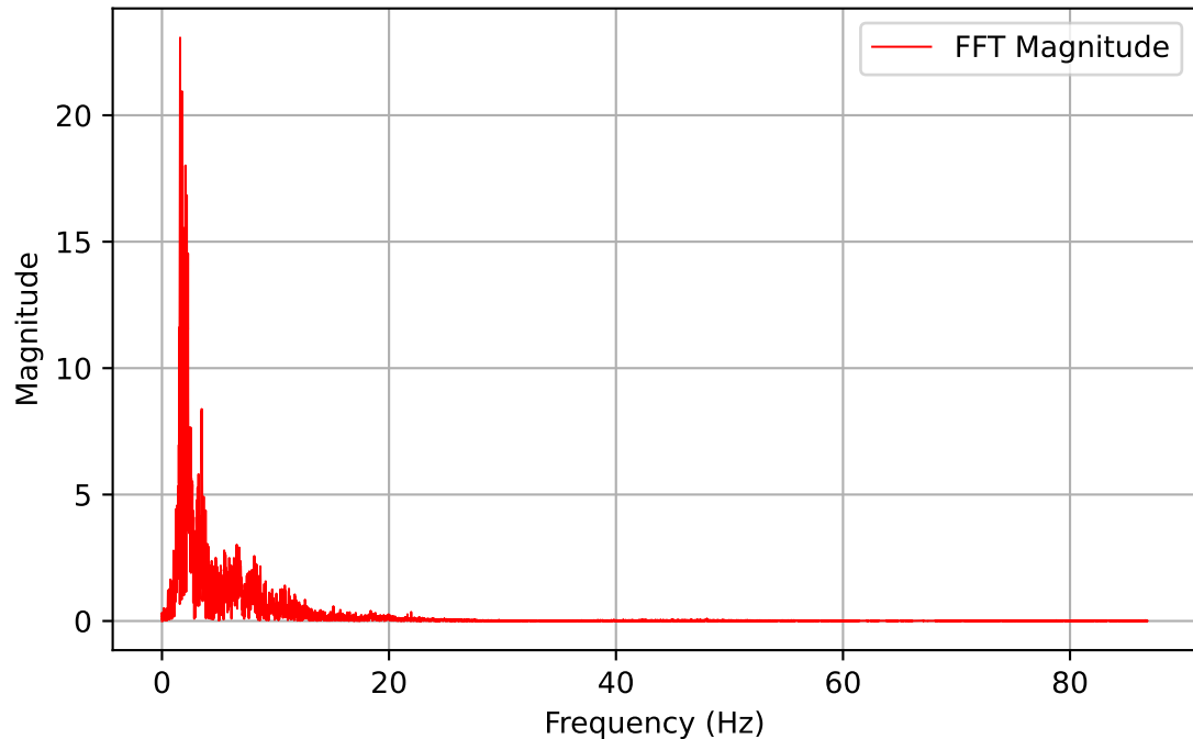
Channel: DYN1-24Y (Frequency Domain)
