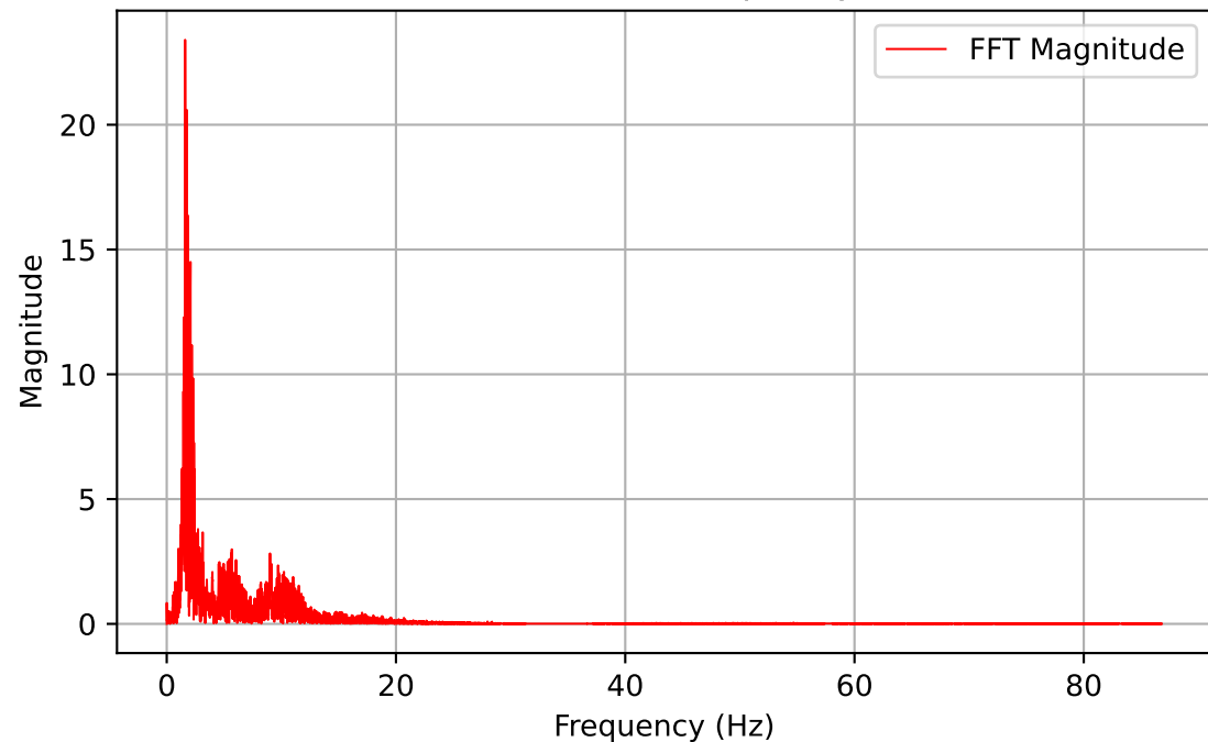
Channel: DYN1-18Y (Frequency Domain)
