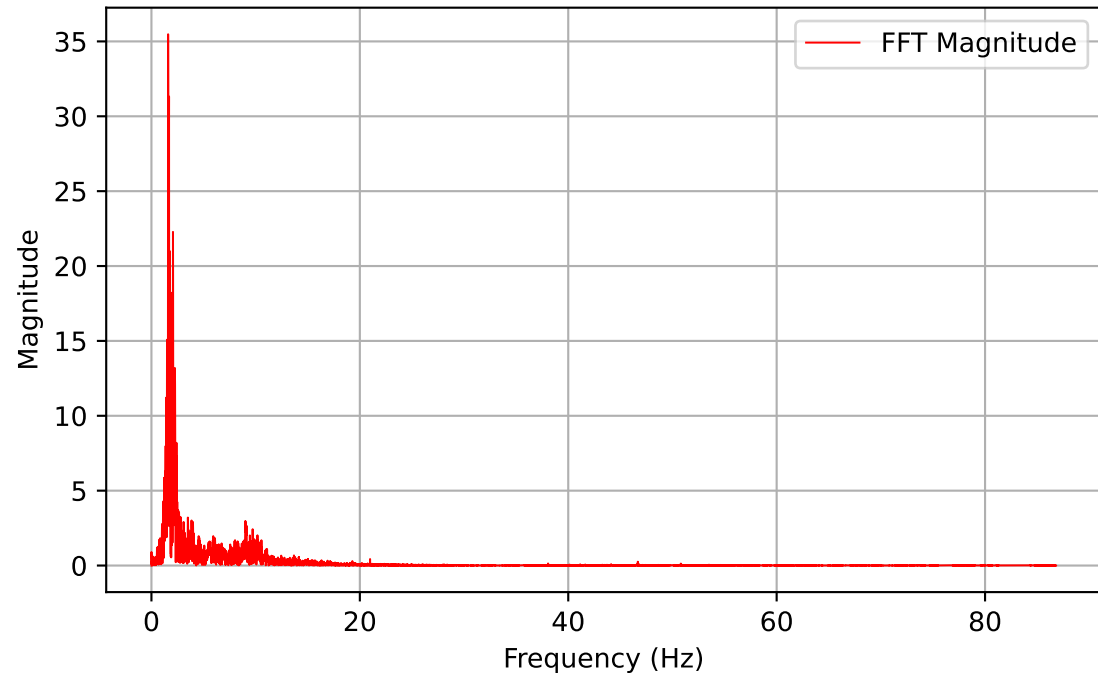
Channel: DYN1-22Y (Frequency Domain)
