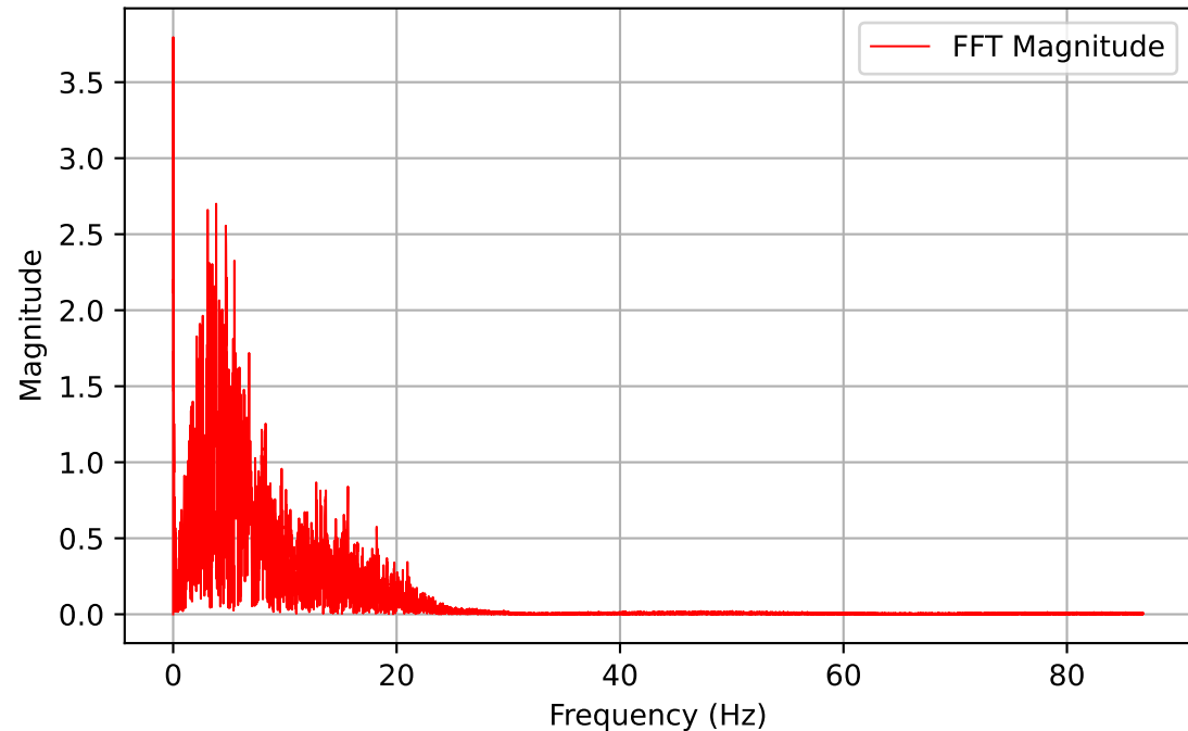
Channel: DYN1-3Y (Frequency Domain)
