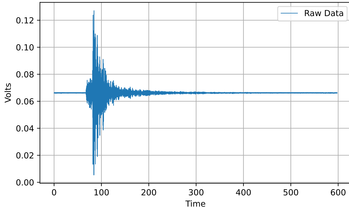
Channel: DYN1-19Y (Time Domain)
