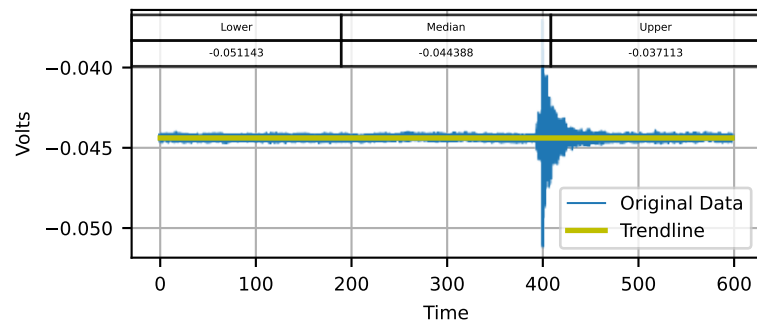
Channel: DYN1-33X (Time Domain)
