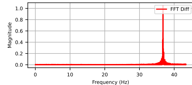
Channel: DYN1-10Y (FFT of Diff)
