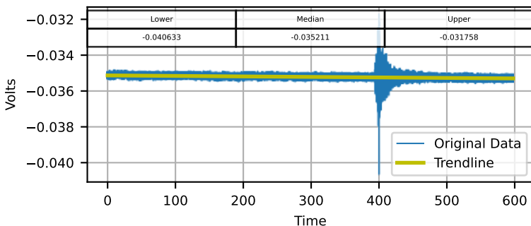
Channel: DYN1-30X (Time Domain)
