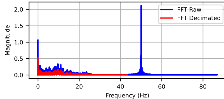
Channel: DYN1-9Y (FFT Overlay)
