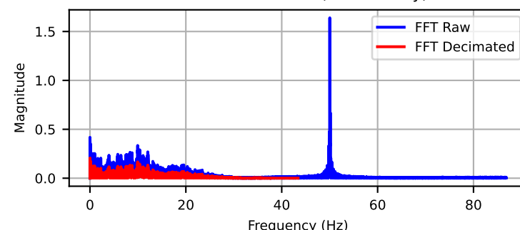
Channel: DYN1-3Y (FFT Overlay)
