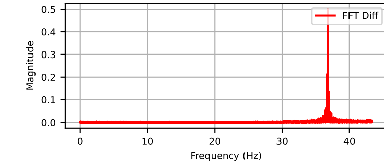
Channel: DYN1-8Y (FFT of Diff)
