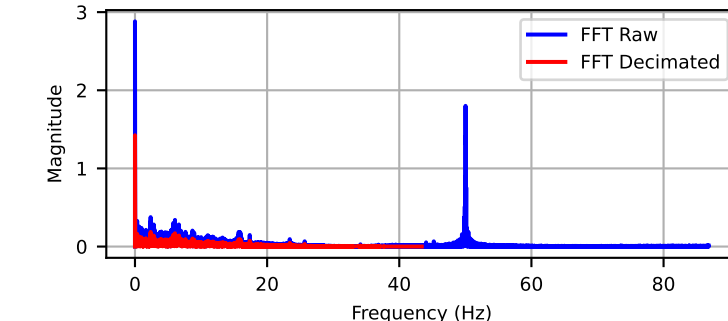
Channel: DYN1-29Y (FFT Overlay)
