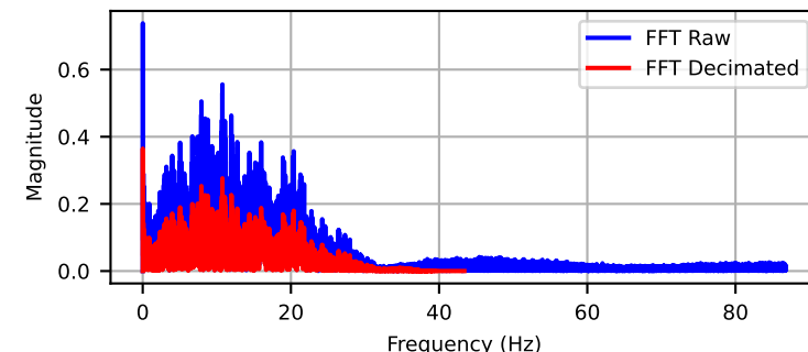
Channel: DYN1-6X (FFT Overlay)
