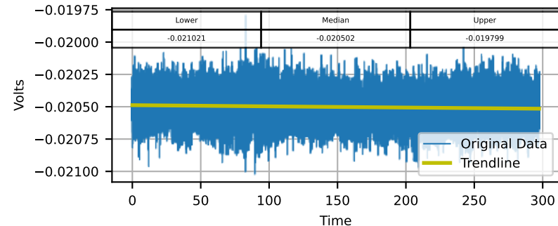
Channel: DYN1-30Y (Time Domain)
