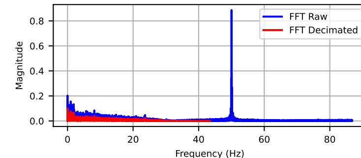
Channel: DYN1-11X (FFT Overlay)
