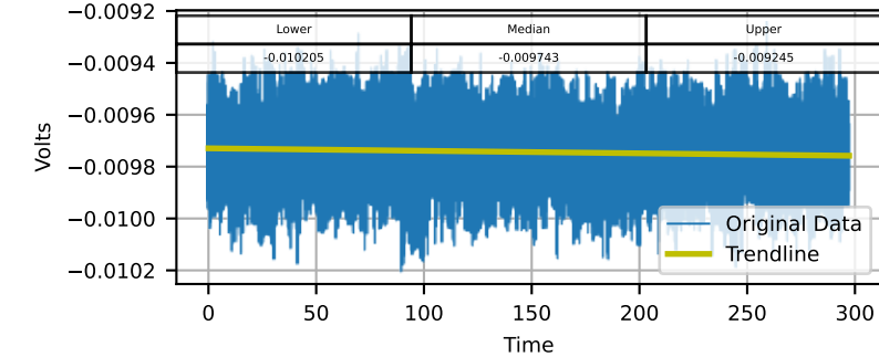
Channel: DYN1-32X (Time Domain)
