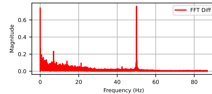
Channel: DYN1-31Y (FFT of Diff)
