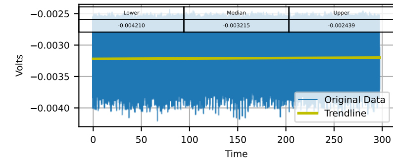
Channel: DYN1-33Y (Time Domain)
