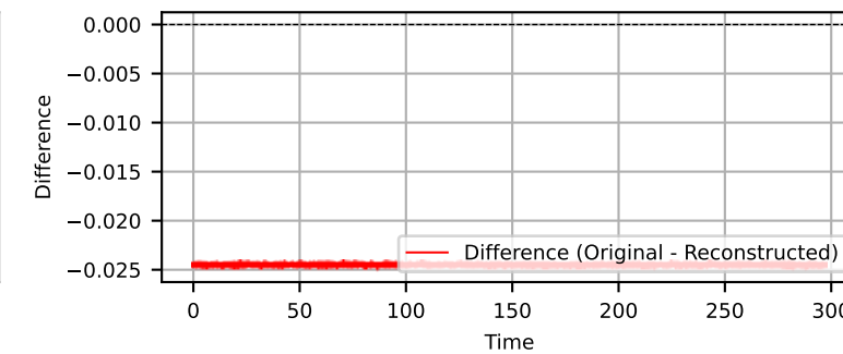
Channel: DYN1-5X (Diff Signal)
