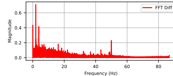
Channel: DYN1-33X (FFT of Diff)
