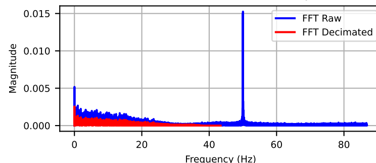
Channel: DYN1-33Y (FFT Overlay)
