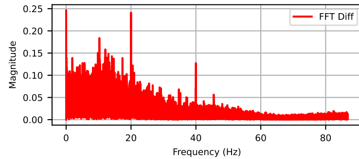
Channel: DYN1-6Y (FFT of Diff)
