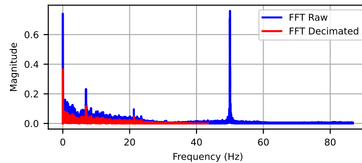
Channel: DYN1-31Y (FFT Overlay)
