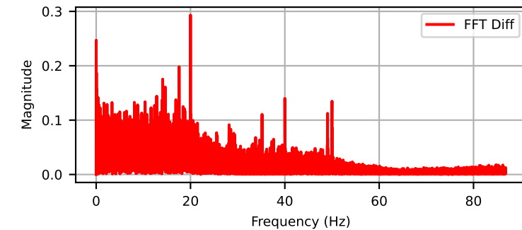
Channel: DYN1-5Y (FFT of Diff)
