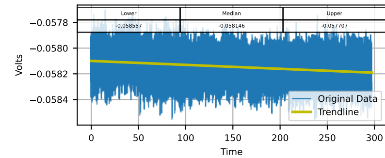
Channel: DYN1-31Y (Time Domain)
