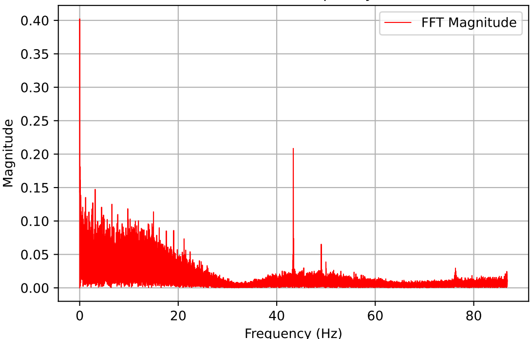
Channel: DYN1-5X (Frequency Domain)
