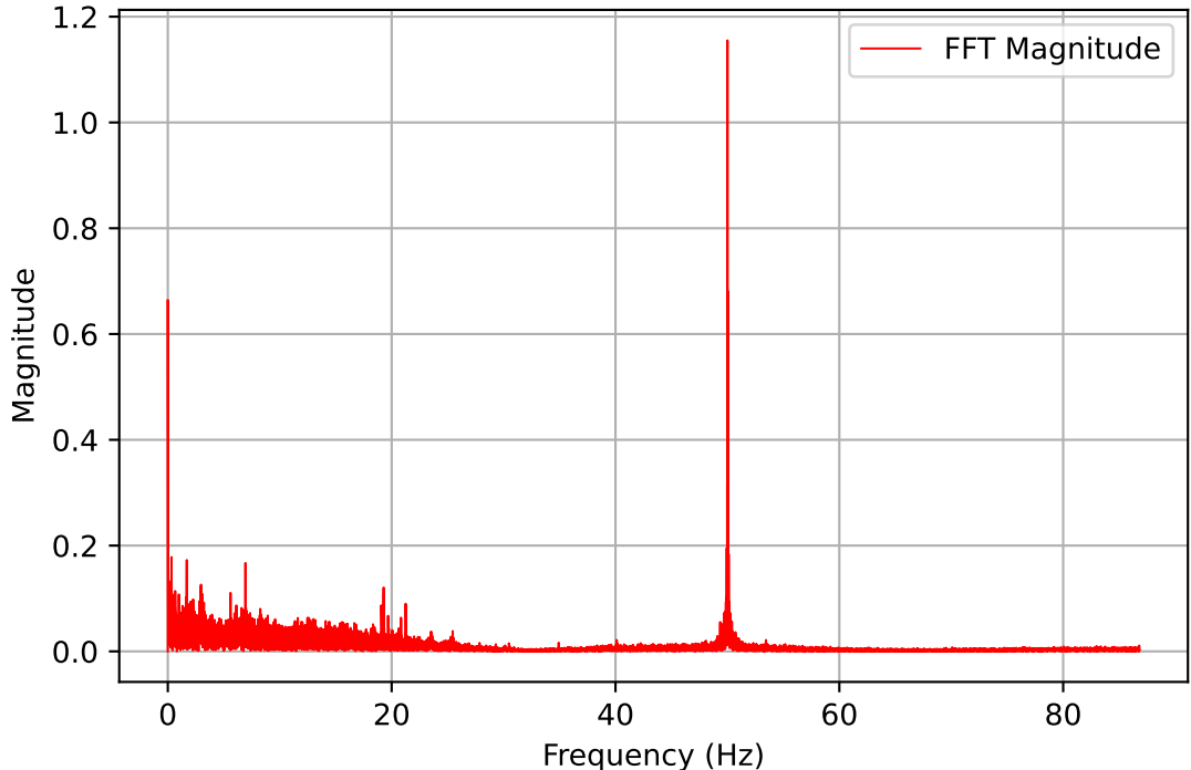
Channel: DYN1-29Y (Frequency Domain)
