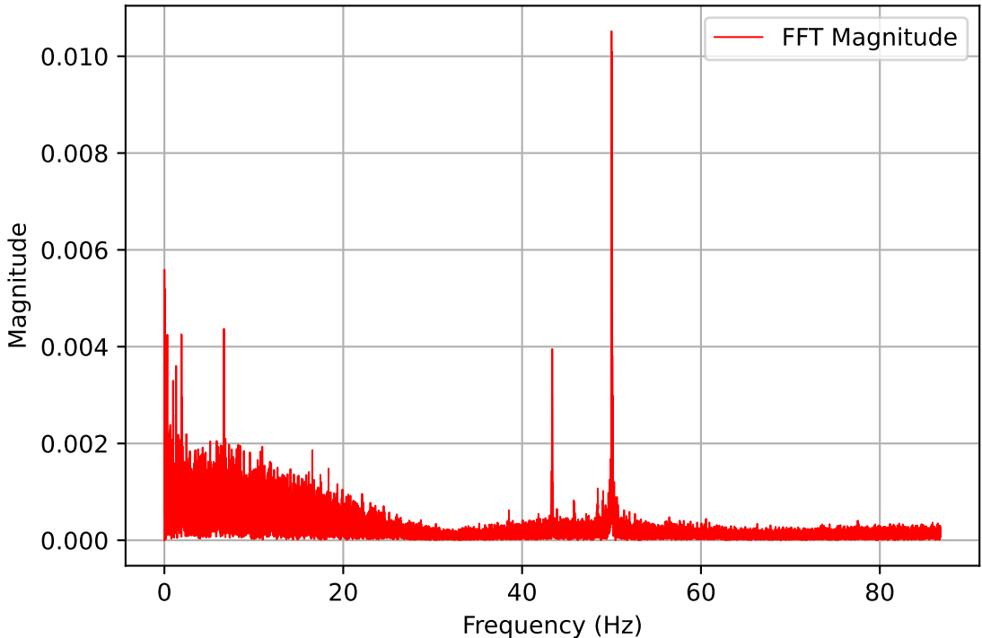
Channel: DYN1-34Y (Frequency Domain)
