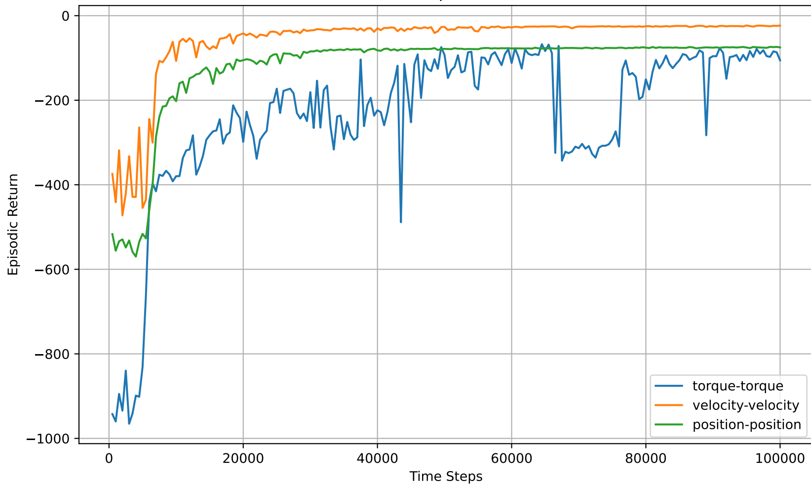
Action-Actuation Episodic Performance
