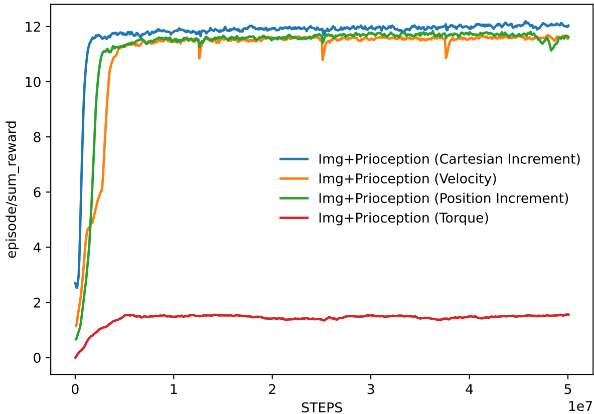
Average Reward
