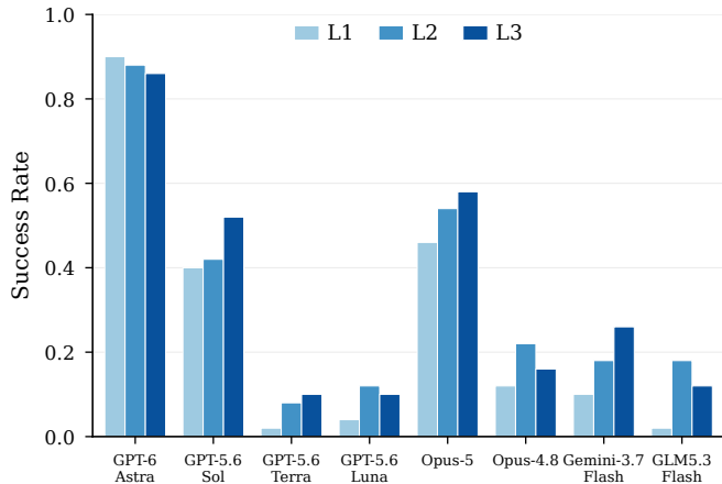
Harness Level and Success Rate
