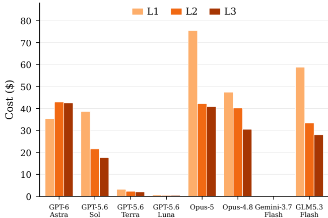
Harness Level and Cost
