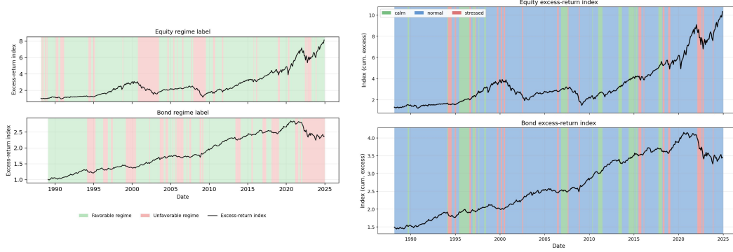
Figure 1: Causal teacher-label representations of the stock–bond history. Both panels report labels formed using information available through the labelled month. Left (INDEPENDENT): equity and bond excess-return indexes with favourable-regime months marked for each leg. Right (COUPLED): cumulative excess-return indexes shaded by calm, normal, and stressed joint regimes.
