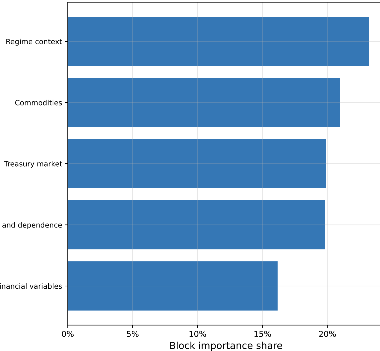
Joint regime — Logistic regression
