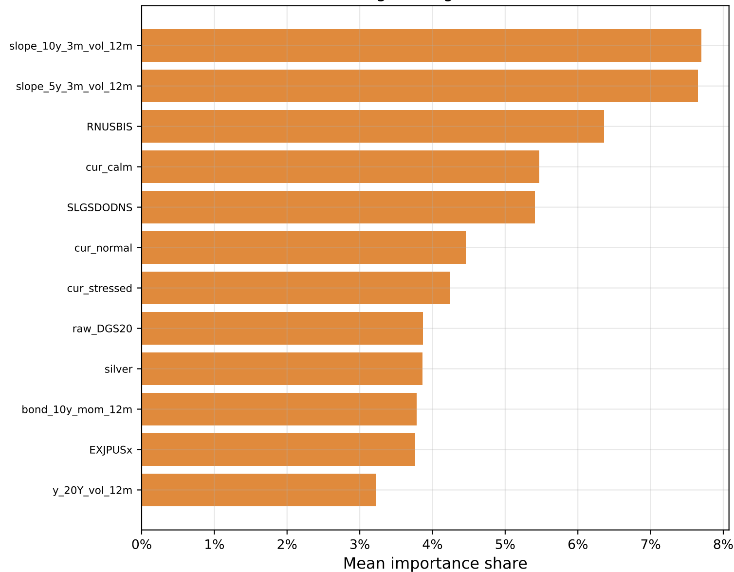
Logistic regression
