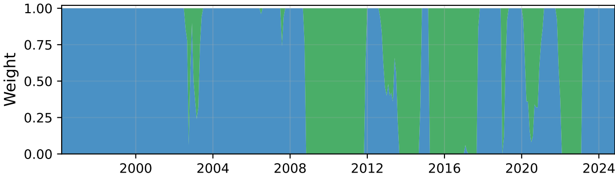
Smoothing half-life 6 Sharpe 0.32; turnover 119%
