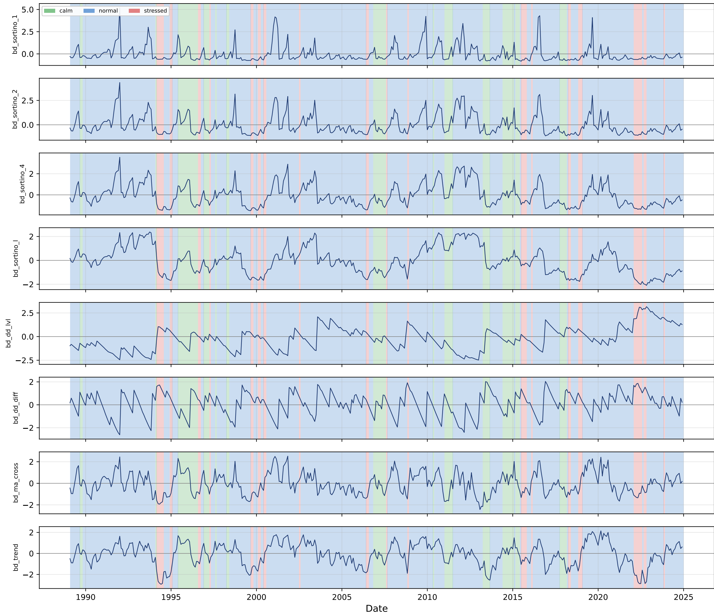
Coupled teacher: bond features (causal rolling z, 120m, 1/99% winsor)
