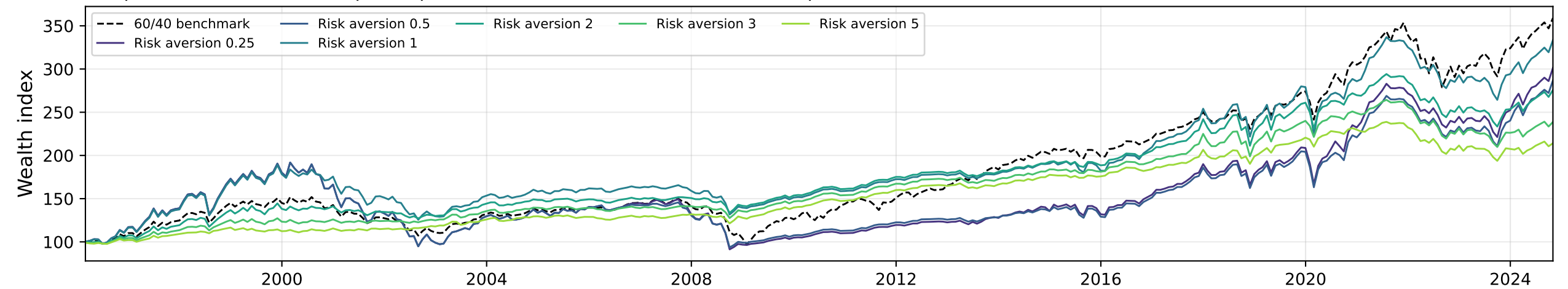
Coupled risk aversion sweep: RF (prob-mixture MV; turnover mult 1, 10 bps)
