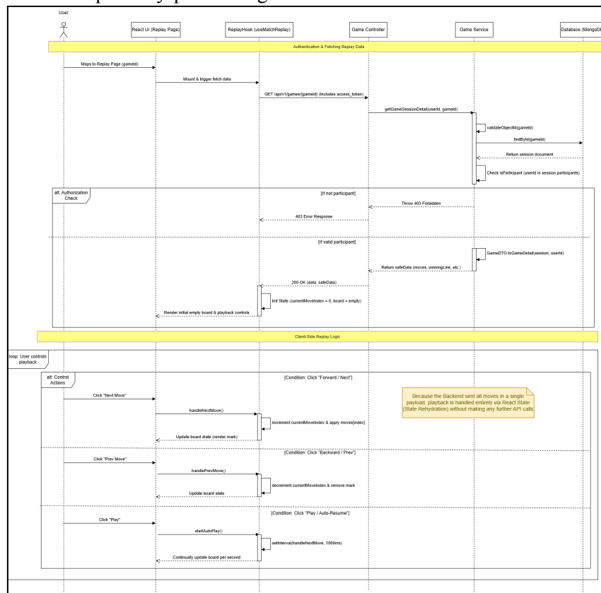
Figure 7: Match Replay Execution Flow [13]
