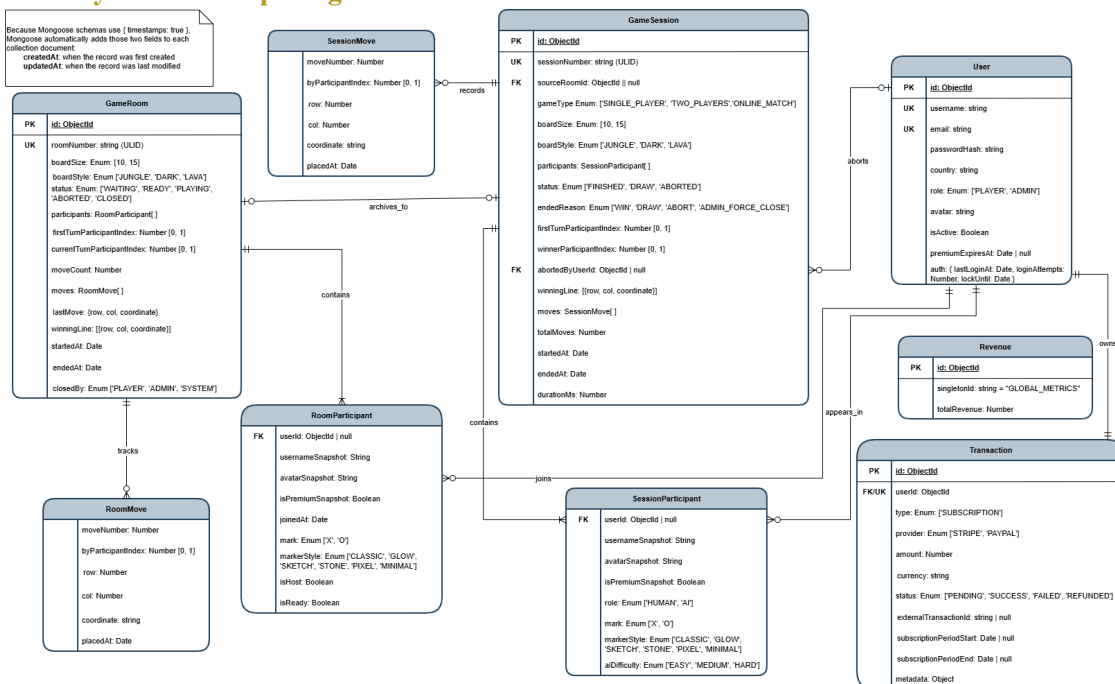
Figure 4: Tictactoang ERD [13]
