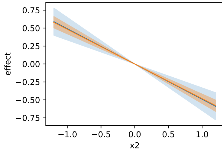
x2: loc
