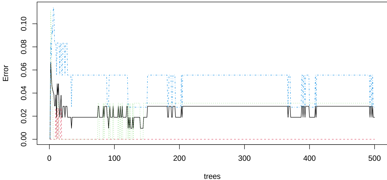
OOB Error vs. Number of Trees
