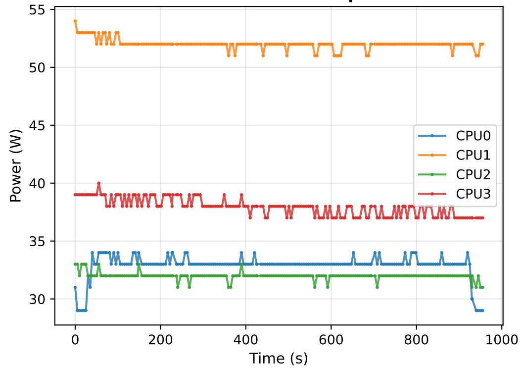
CPU Power Consumption
