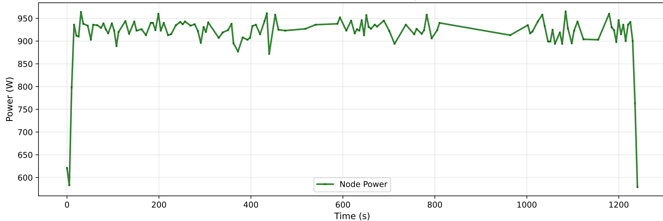
Total Node Power Consumption
