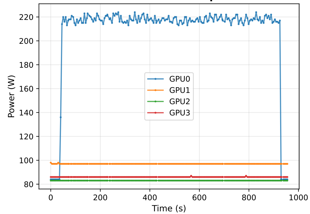
GPU Power Consumption
