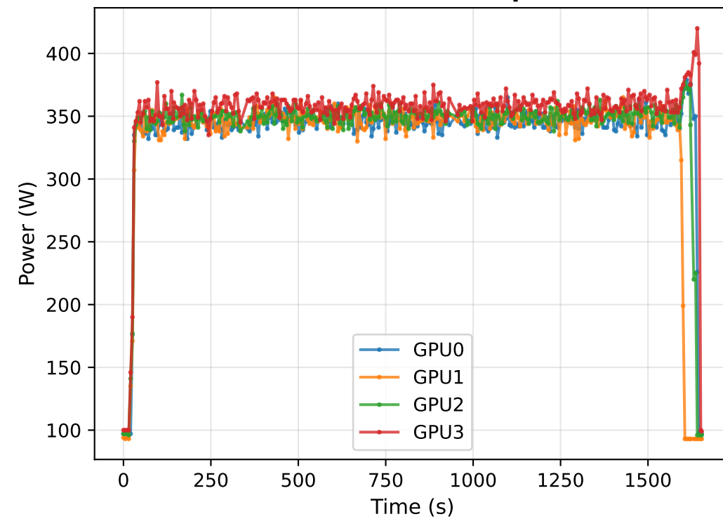
GPU Power Consumption
