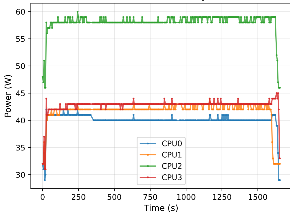
CPU Power Consumption
