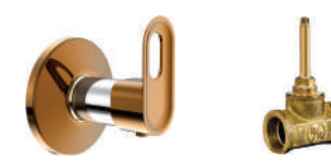
CONCEALED FLUSH COCK BODY IN 25 MM CARTRIDGE (SUITABLE FOR 25 MM PIPELINE)
