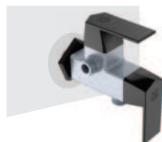
2 IN 1 ANGLE COCK WITH FLANGE ART NO. RNG2009B15 MRP : ₹532/-
