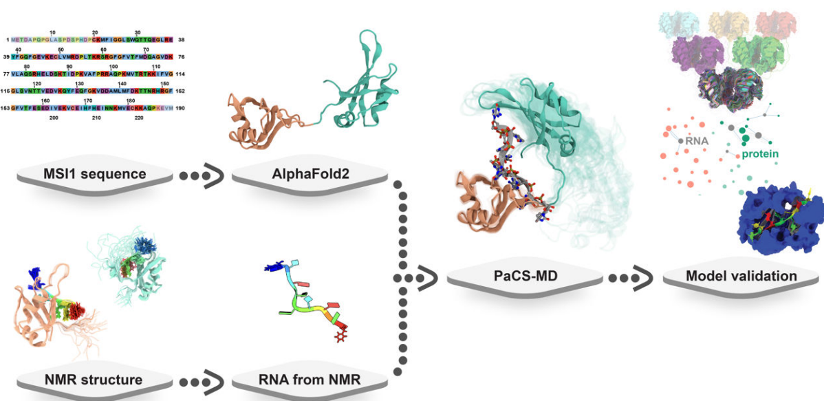
Figure 1. Workflow of an efficient structural refinement technique for protein-RNA complexes based on a combination of AI-based modeling (AlphaFold2) and flexible docking (PaCS-MD). Initially, AI-based modeling of protein-RNA structures is conducted with AlphaFold2. Subsequently, experimental data provides RNA/protein recognition site information, which is incorporated into the model. PaCS-MD is then employed to generate a variety of protein-RNA complexes based on flexible docking. Finally, the structural validation of protein-RNA complexes is performed through MD simulation, end-point binding free energy calculation, and interaction network analysis described by the orange and blue circles in the top right corner of the workflow.
