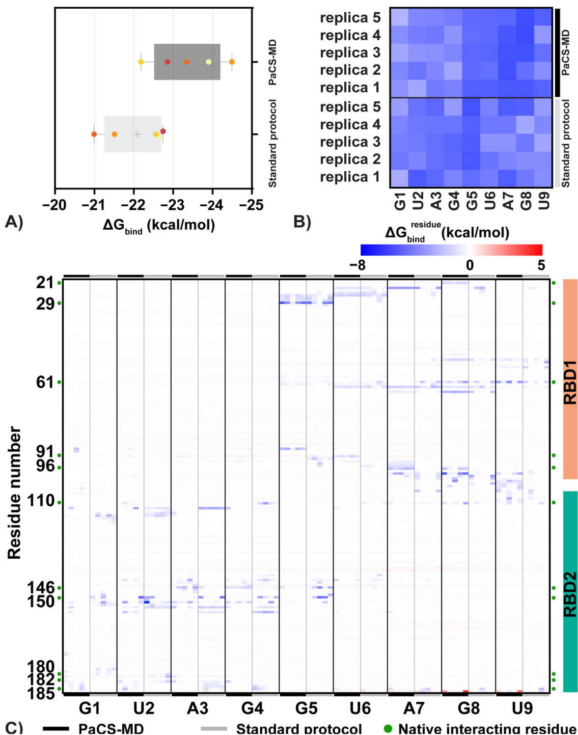
Figure 3. (A) \Delta G_{\text{bind}} averaged over the five replicas of both PaCS-MD and Phyre2. (B) \Delta G_{\text{bind}}^{\text{residue}} of the five replicas of both protocols versus the target sequence (5'-GUAGGUAGU-3'). (C) The decomposition of \Delta G_{\text{bind}} into amino-acid residues and RNA units. The native interacting residues in the NMR structures of RBD1 and RBD2 are highlighted by green dots. The same spectrum bar is used for both (B) and (C).
