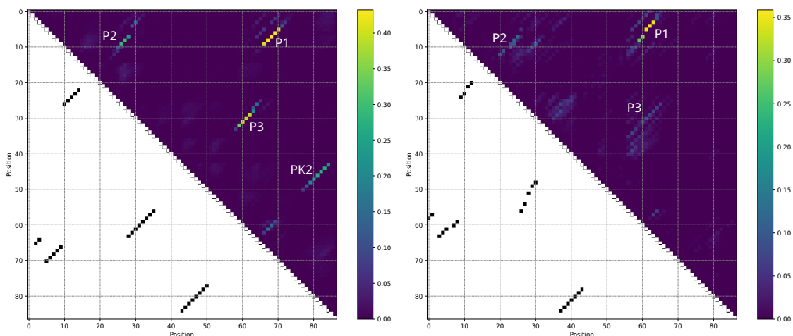
Figure S7: Comparison between Infrared and cmemit designs. Base-pairing probability matrices for sequences designed with the Infrared model (left) and the MBFV covariance model (right). Probabilities were obtained by averaging base pairing probabilities across all designs within each set. The upper triangles show the averaged pairing probabilities with annotated structural elements (P1, P2, P3, PK2), whereas the lower triangles show the corresponding target structure.
