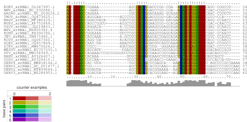
Figure S1: Structural multiple sequence alignment of natural xrRNAs. Structural alignment and consensus secondary structure of natural xrRNA sequences from representative MBFV isolates calculated with mLocARNA. Square brackets depict pseudoknot interactions of PK1. PK2 is not predicted in this consensus structure.
