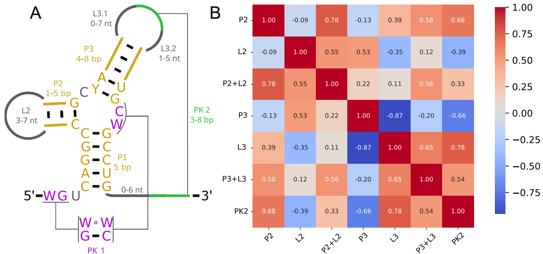
Figure S2: Length correlations between xrRNA structural elements. A. Symbolic representation of the structural diversity of MBFV xrRNAs. Conserved elements are highlighted in ochre (stems P1-P3), grey (loops L2 and L3), and purple/green (Pseudoknots PK1 and PK2). Positions with >90 % sequence conservation are shown using IUPAC nucleotide symbols. B. Pearson correlation coefficients quantifying the association between the lengths of conserved structural elements in the selected MBFV xrRNA sequences.
