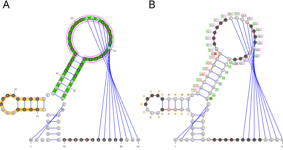
Figure S3: Visualization of the Infrared model. A. Variables used in the design model. Position-specific domains are indicated using IUPAC nucleotide codes; the additional symbol X denotes the extended domain \{A, C, G, U, \epsilon\} . A red backbone marks regions subject to a unique sequence constraint, whereas colored outlines indicate length-correlation constraints between regions. B. Variable assignment for the MBFV model corresponding to the design syn-xrRNA1. Auxiliary variables used to count region lengths are shown adjacent to the base positions as color-coded squares. The terminal variable representing the total length of each region is highlighted as a filled square.
