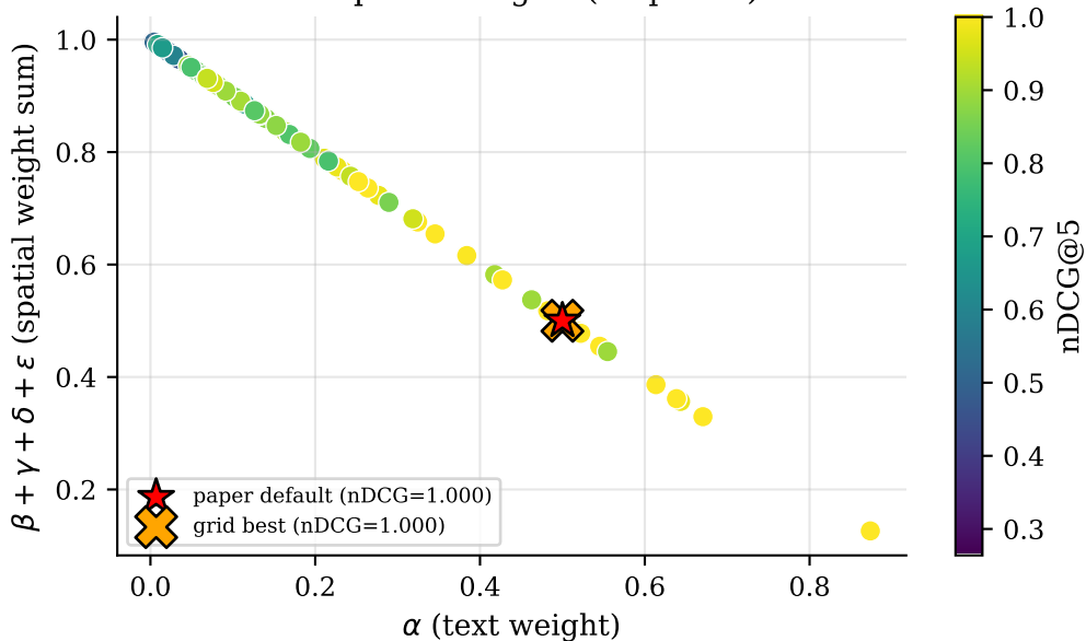
5-simplex LHS grid (81 points)
